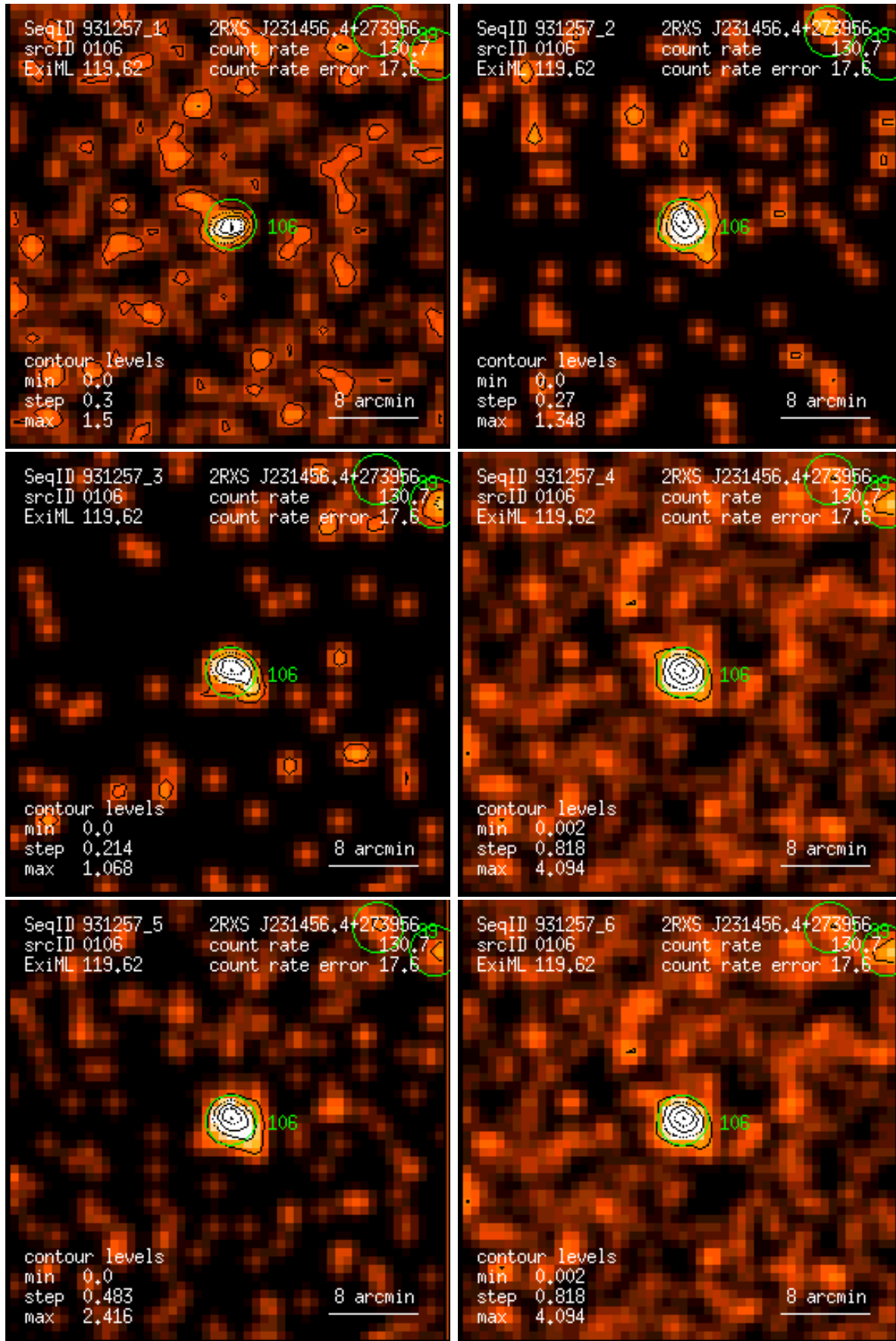
Figure 106: RASS 931257: detection 0106: band rate images, Gaussian filter: (1) PSPC channels 11 – 41, (2) 52 – 90, (3) 91 – 201, (4) 11 – 235, (5) 52 – 201, (6) 11 – 201. Broad band rates in counts/ks. Band rate contour levels in counts/ks/arcmin 2 .
