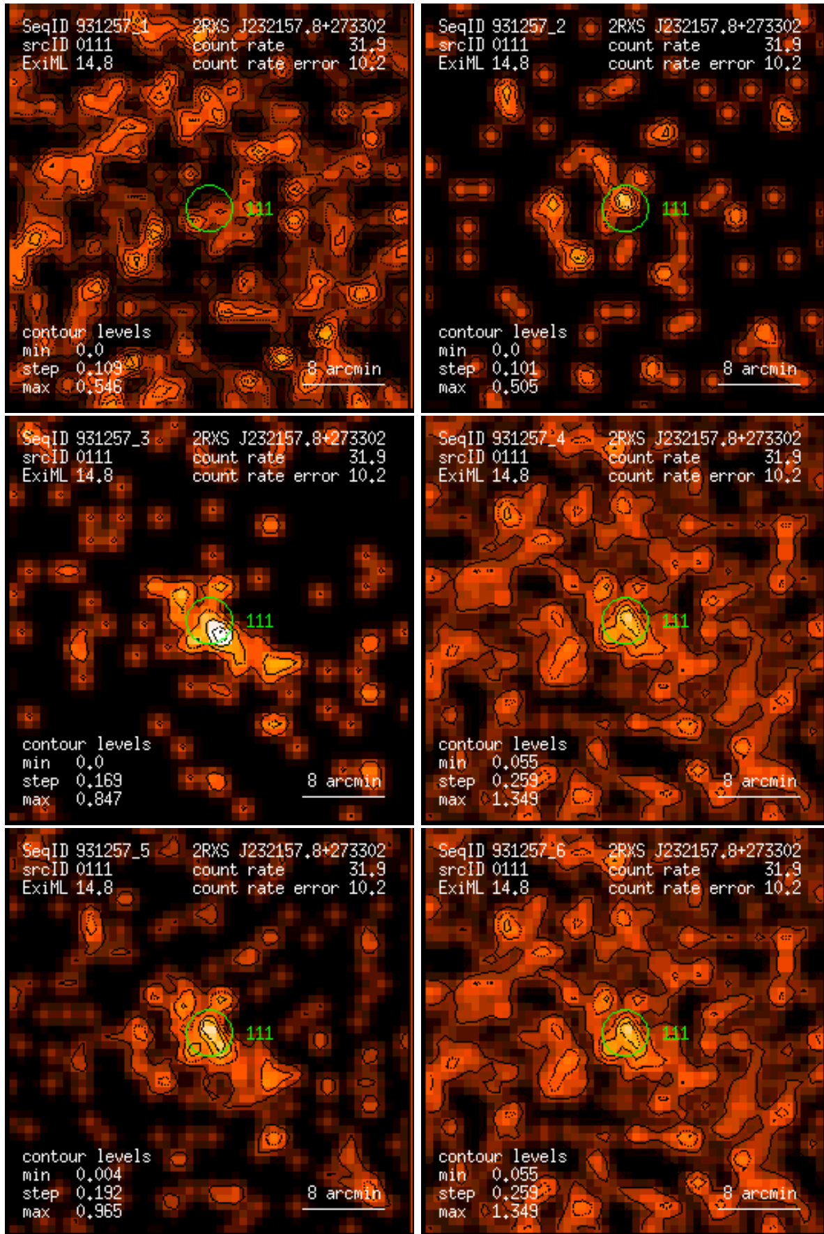
Figure 111: RASS 931257: detection 0111: band rate images, Gaussian filter: (1) PSPC channels 11 – 41, (2) 52 – 90, (3) 91 – 201, (4) 11 – 235, (5) 52 – 201, (6) 11 – 201. Broad band rates in counts/ks. Band rate contour levels in counts/ks/arcmin 2 .
