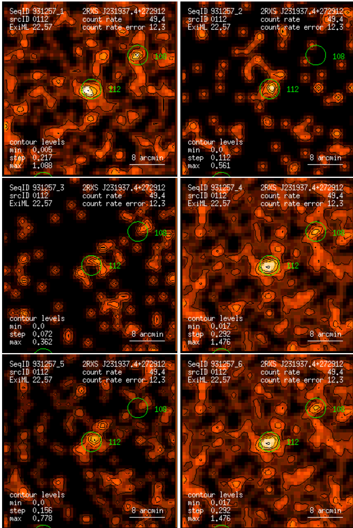
Figure 112: RASS 931257: detection 0112: band rate images, Gaussian filter: (1) PSPC channels 11 – 41, (2) 52 – 90, (3) 91 – 201, (4) 11 – 235, (5) 52 – 201, (6) 11 – 201. Broad band rates in counts/ks. Band rate contour levels in counts/ks/arcmin 2 .
