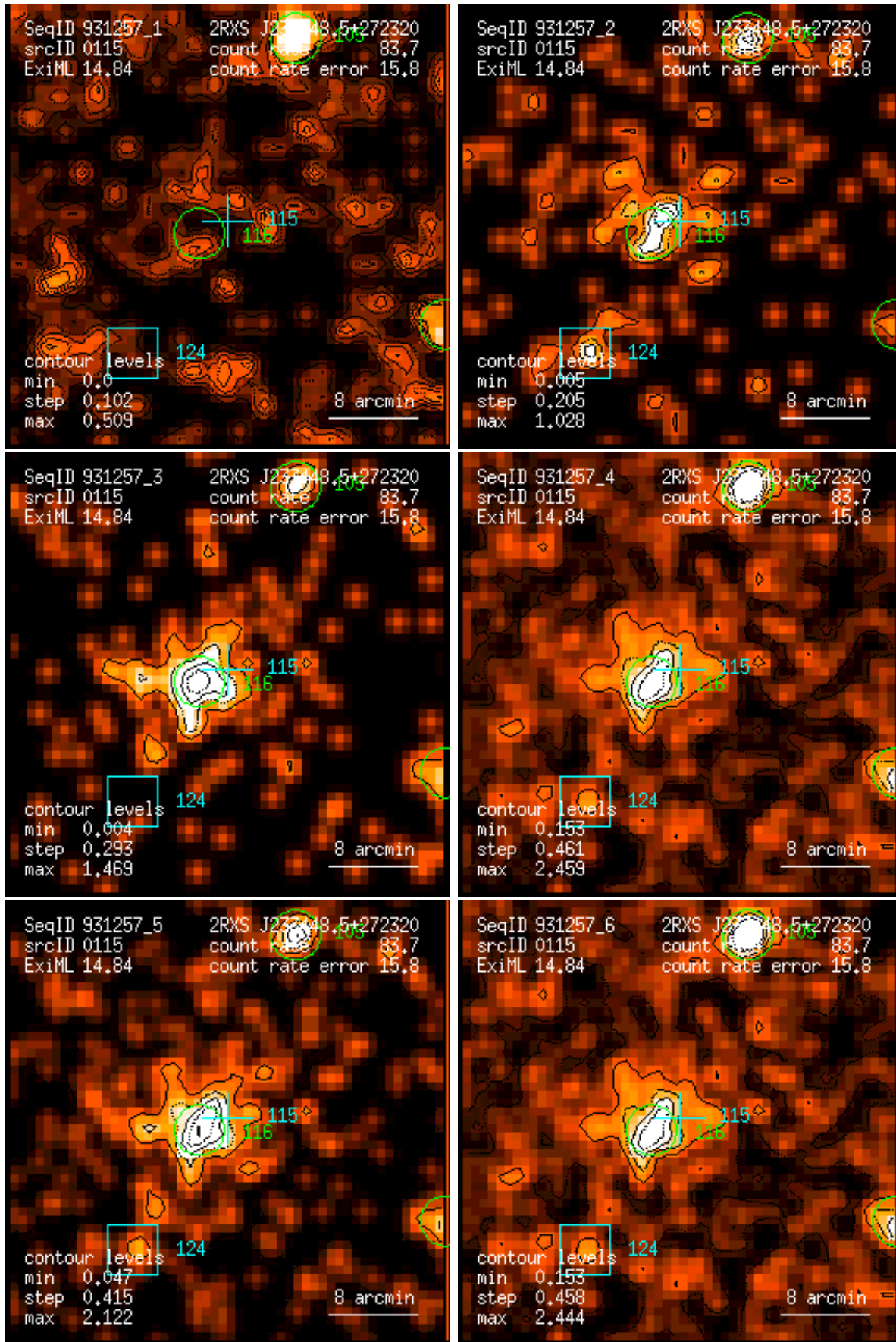
Figure 115: RASS 931257: detection 0115: band rate images, Gaussian filter: (1) PSPC channels 11 – 41, (2) 52 – 90, (3) 91 – 201, (4) 11 – 235, (5) 52 – 201, (6) 11 – 201. Broad band rates in counts/ks. Band rate contour levels in counts/ks/arcmin 2 .
