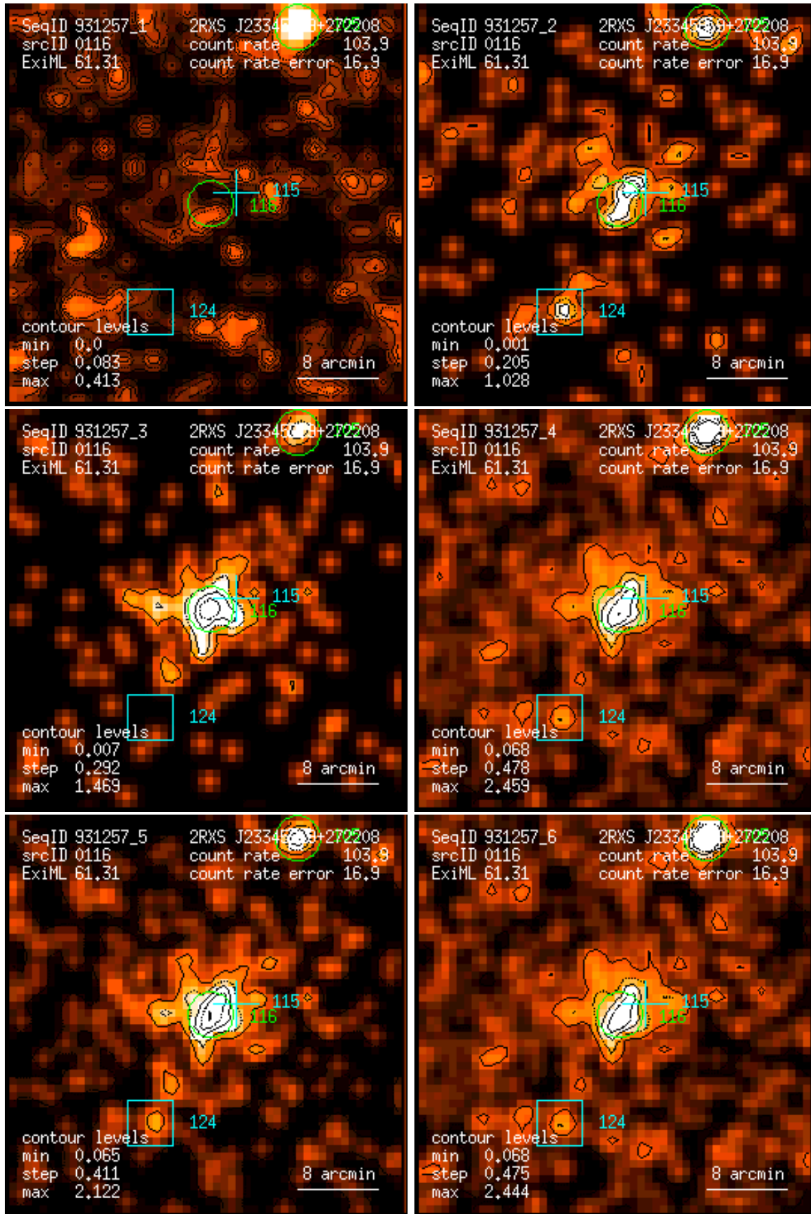
Figure 116: RASS 931257: detection 0116: band rate images, Gaussian filter: (1) PSPC channels 11 – 41, (2) 52 – 90, (3) 91 – 201, (4) 11 – 235, (5) 52 – 201, (6) 11 – 201. Broad band rates in counts/ks. Band rate contour levels in counts/ks/arcmin 2 .
