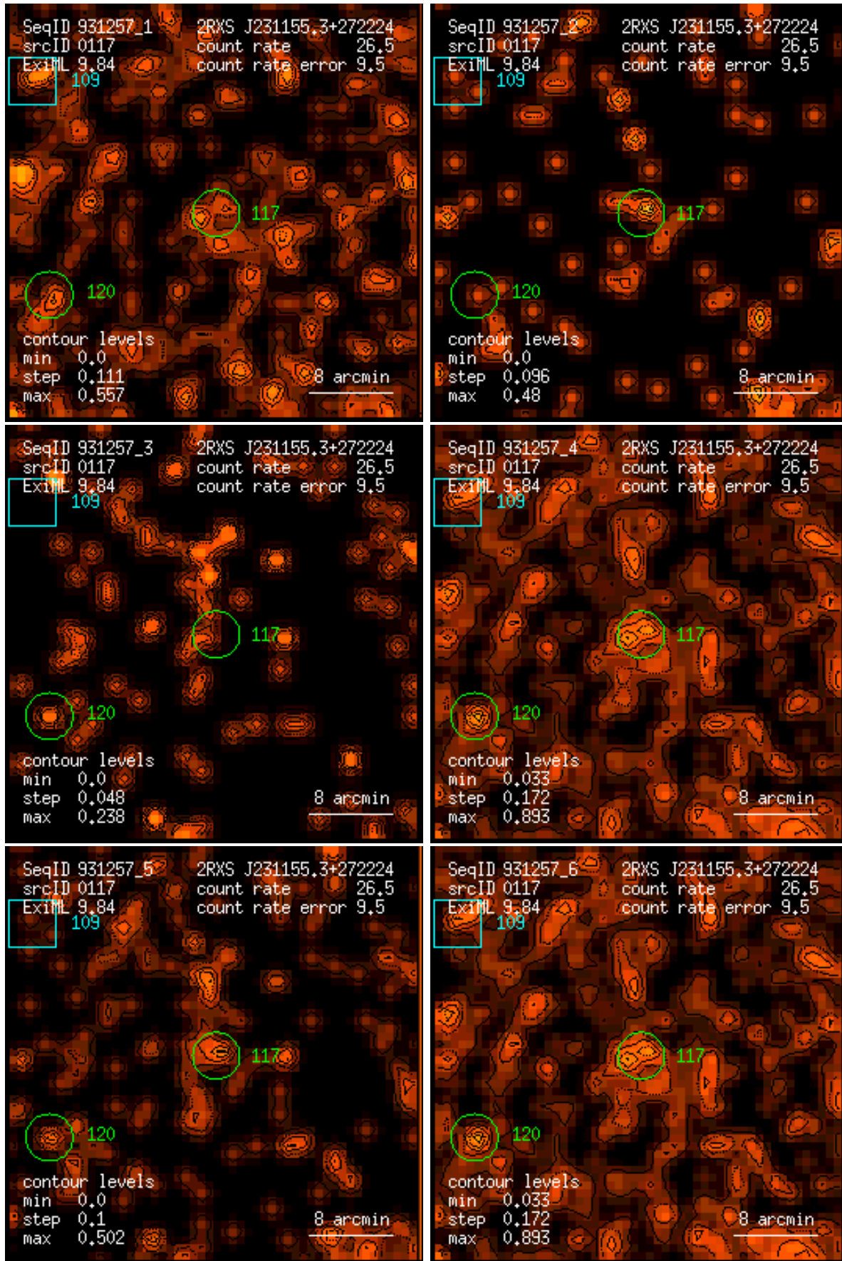
Figure 117: RASS 931257: detection 0117: band rate images, Gaussian filter: (1) PSPC channels 11 – 41, (2) 52 – 90, (3) 91 – 201, (4) 11 – 235, (5) 52 – 201, (6) 11 – 201. Broad band rates in counts/ks. Band rate contour levels in counts/ks/arcmin 2 .
