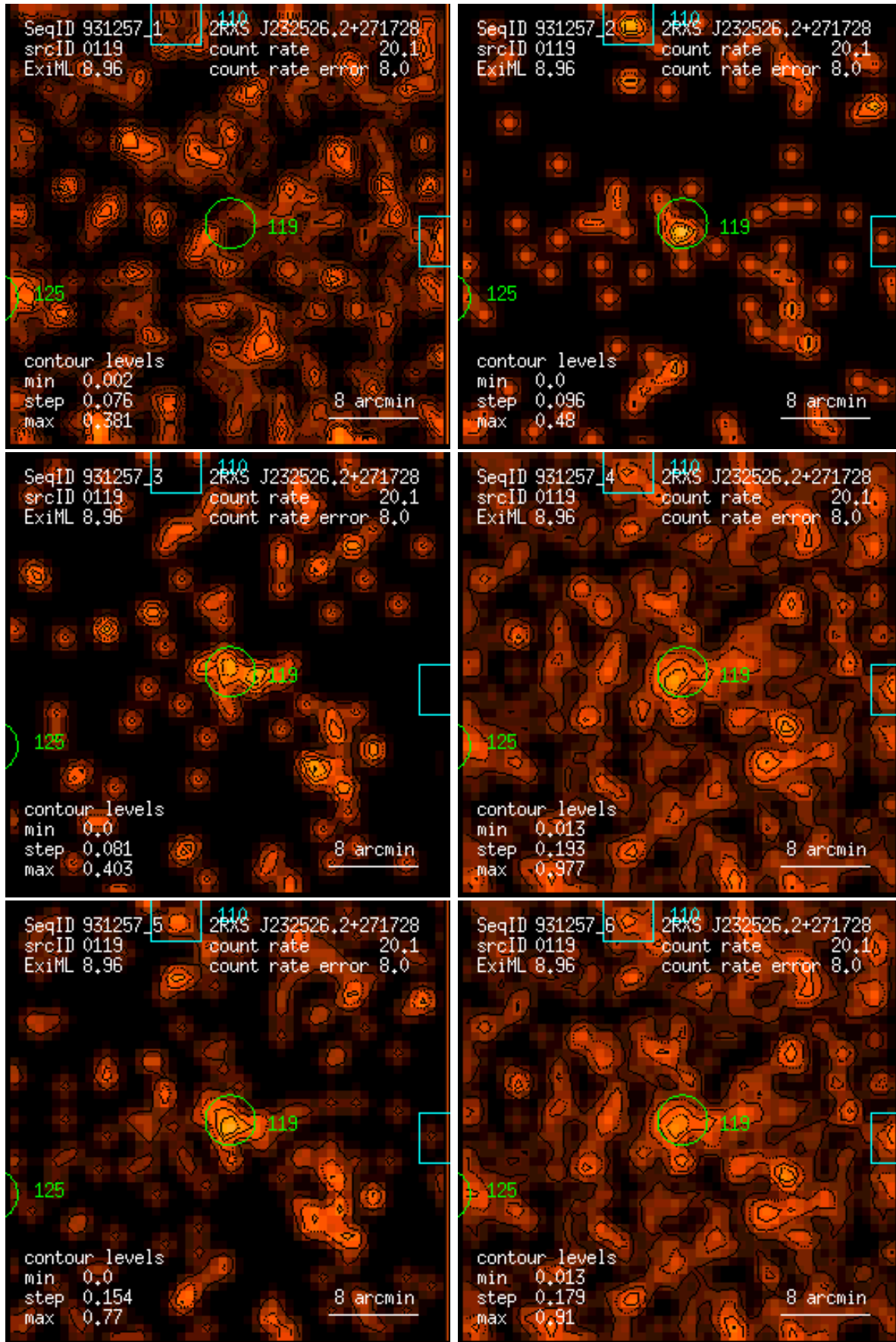
Figure 119: RASS 931257: detection 0119: band rate images, Gaussian filter: (1) PSPC channels 11 – 41, (2) 52 – 90, (3) 91 – 201, (4) 11 – 235, (5) 52 – 201, (6) 11 – 201. Broad band rates in counts/ks. Band rate contour levels in counts/ks/arcmin 2 .
