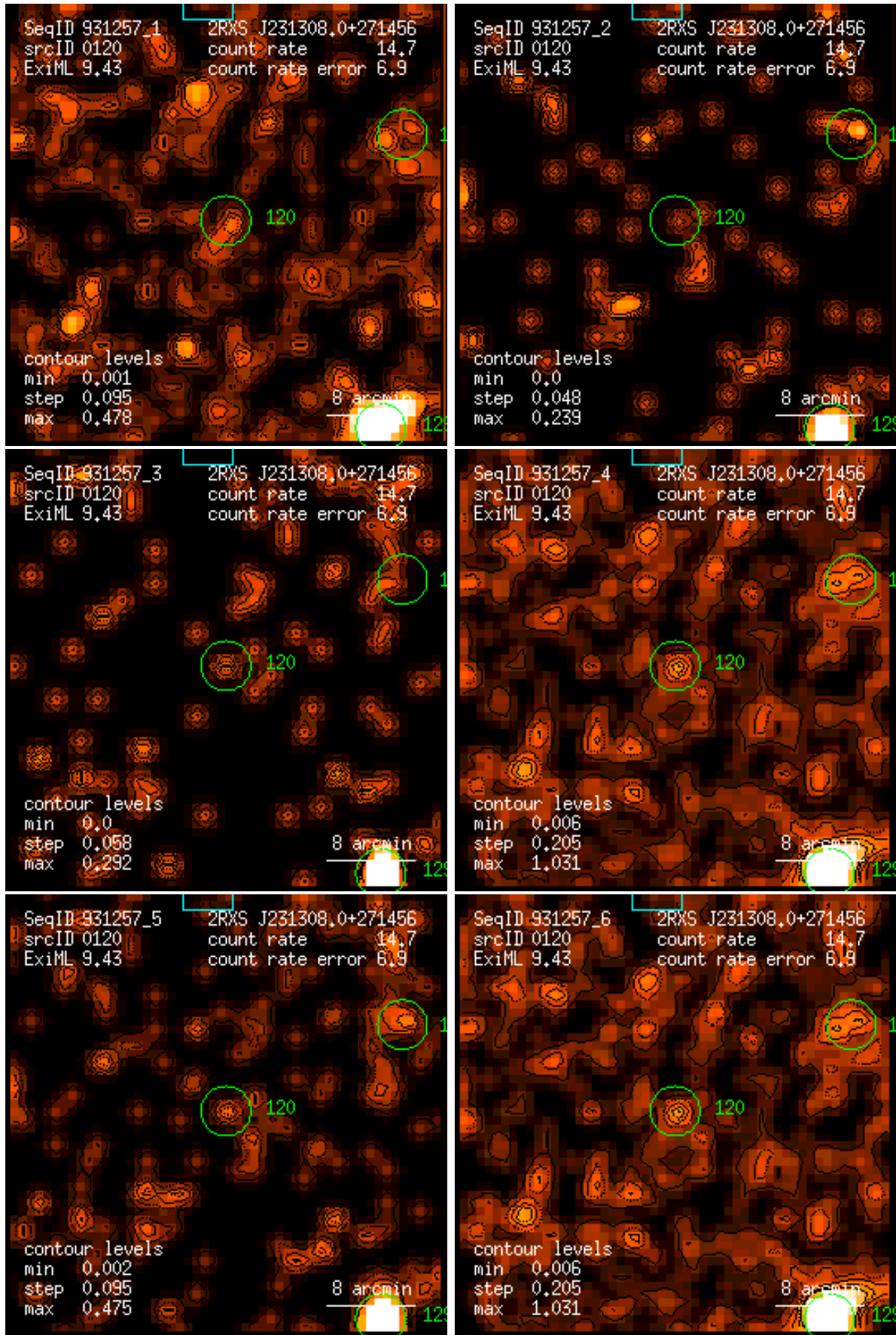
Figure 120: RASS 931257: detection 0120: band rate images, Gaussian filter: (1) PSPC channels 11 – 41, (2) 52 – 90, (3) 91 – 201, (4) 11 – 235, (5) 52 – 201, (6) 11 – 201. Broad band rates in counts/ks. Band rate contour levels in counts/ks/arcmin 2 .
