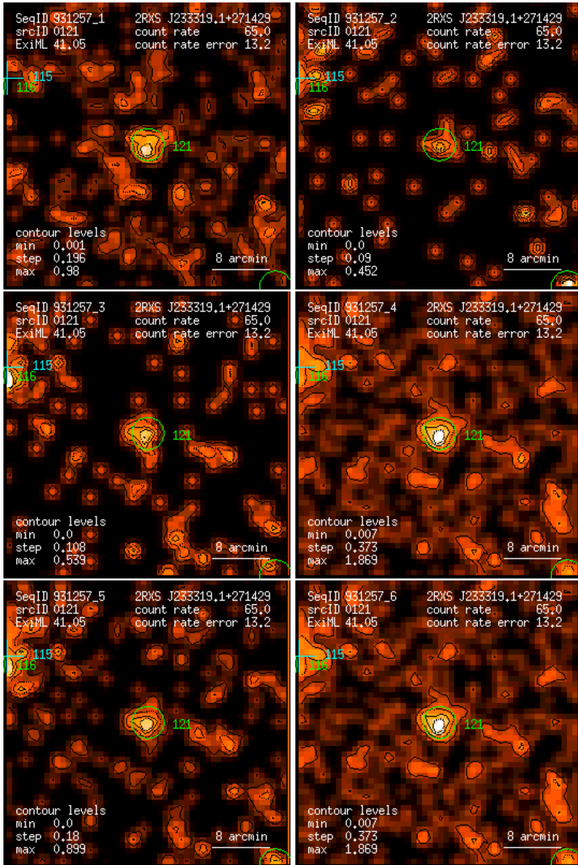
Figure 121: RASS 931257: detection 0121: band rate images, Gaussian filter: (1) PSPC channels 11 – 41, (2) 52 – 90, (3) 91 – 201, (4) 11 – 235, (5) 52 – 201, (6) 11 – 201. Broad band rates in counts/ks. Band rate contour levels in counts/ks/arcmin 2 .
