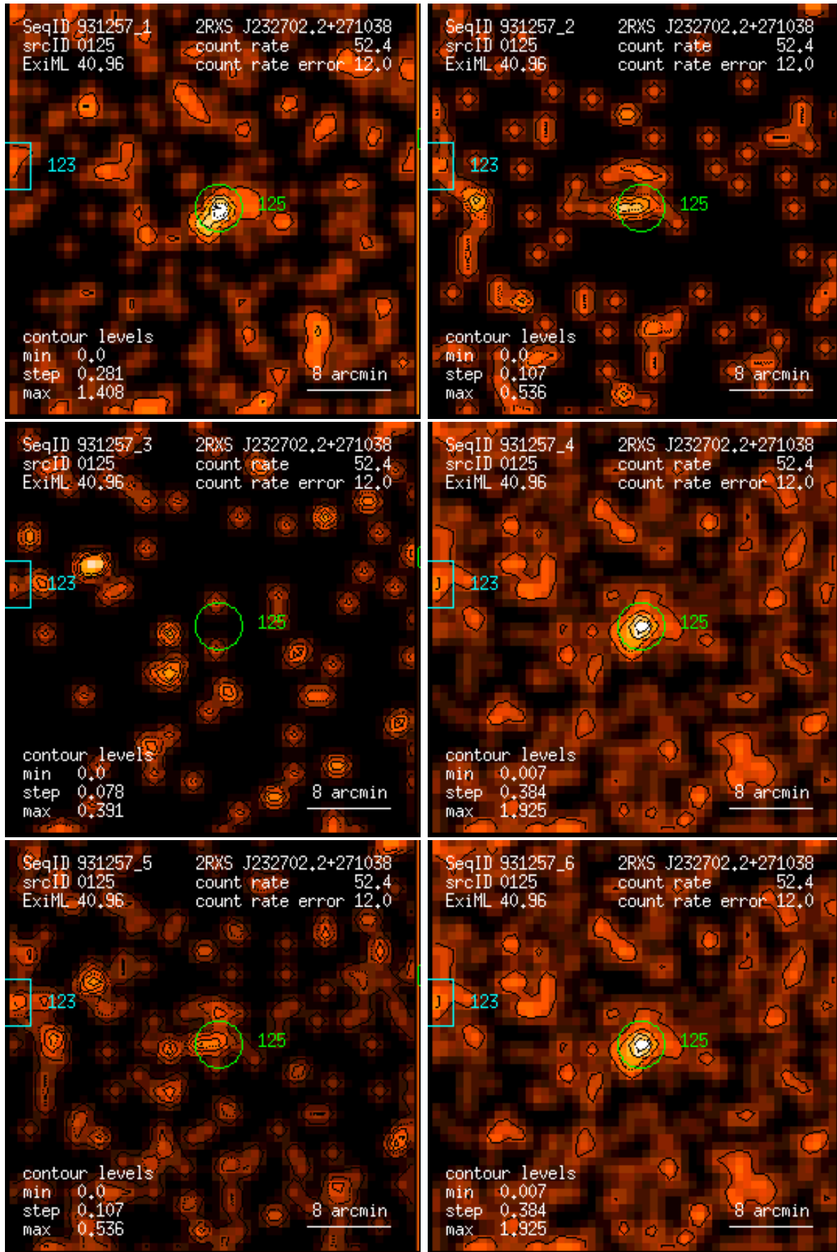
Figure 125: RASS 931257: detection 0125: band rate images, Gaussian filter: (1) PSPC channels 11 – 41, (2) 52 – 90, (3) 91 – 201, (4) 11 – 235, (5) 52 – 201, (6) 11 – 201. Broad band rates in counts/ks. Band rate contour levels in counts/ks/arcmin 2 .
