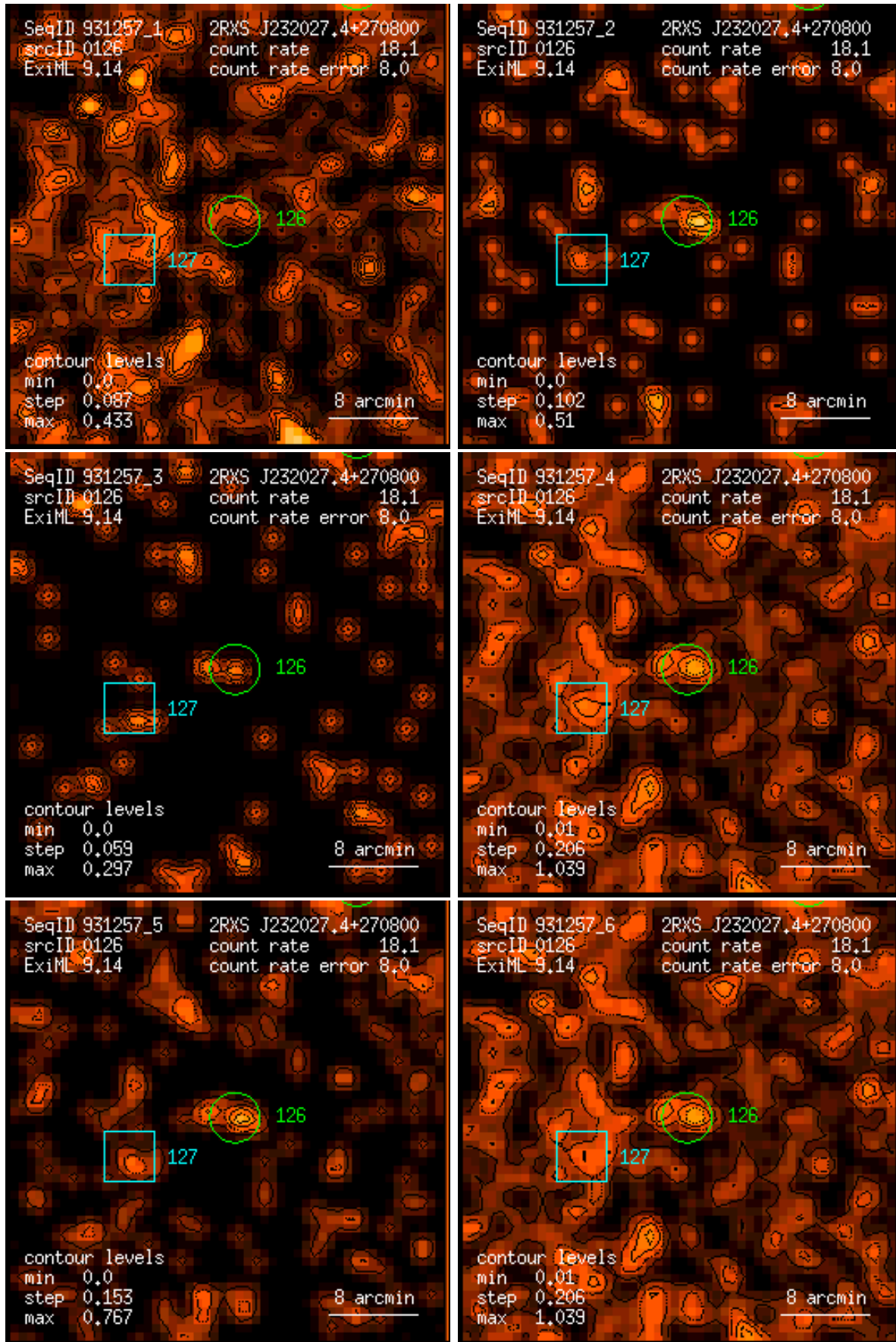
Figure 126: RASS 931257: detection 0126: band rate images, Gaussian filter: (1) PSPC channels 11 – 41, (2) 52 – 90, (3) 91 – 201, (4) 11 – 235, (5) 52 – 201, (6) 11 – 201. Broad band rates in counts/ks. Band rate contour levels in counts/ks/arcmin 2 .
