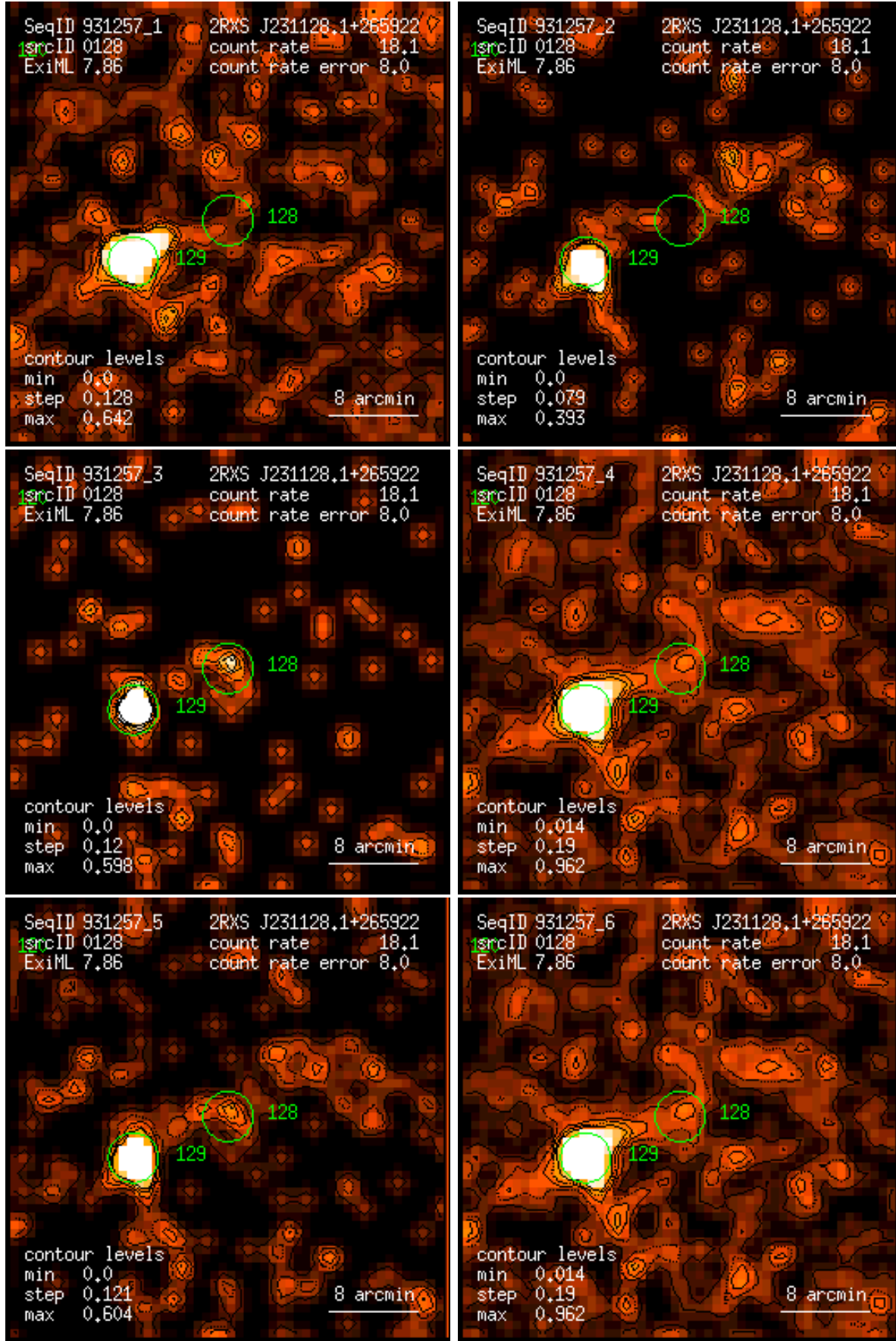
Figure 128: RASS 931257: detection 0128: band rate images, Gaussian filter: (1) PSPC channels 11 – 41, (2) 52 – 90, (3) 91 – 201, (4) 11 – 235, (5) 52 – 201, (6) 11 – 201. Broad band rates in counts/ks. Band rate contour levels in counts/ks/arcmin 2 .
