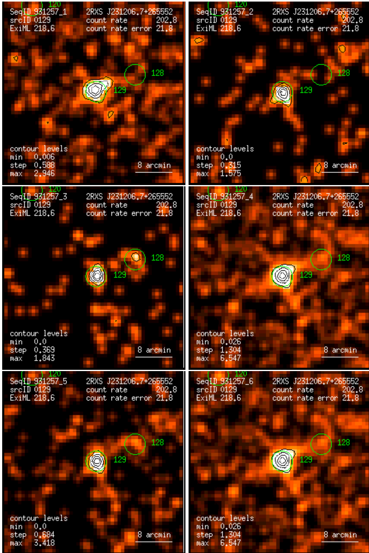
Figure 129: RASS 931257: detection 0129: band rate images, Gaussian filter: (1) PSPC channels 11 – 41, (2) 52 – 90, (3) 91 – 201, (4) 11 – 235, (5) 52 – 201, (6) 11 – 201. Broad band rates in counts/ks. Band rate contour levels in counts/ks/arcmin 2 .
