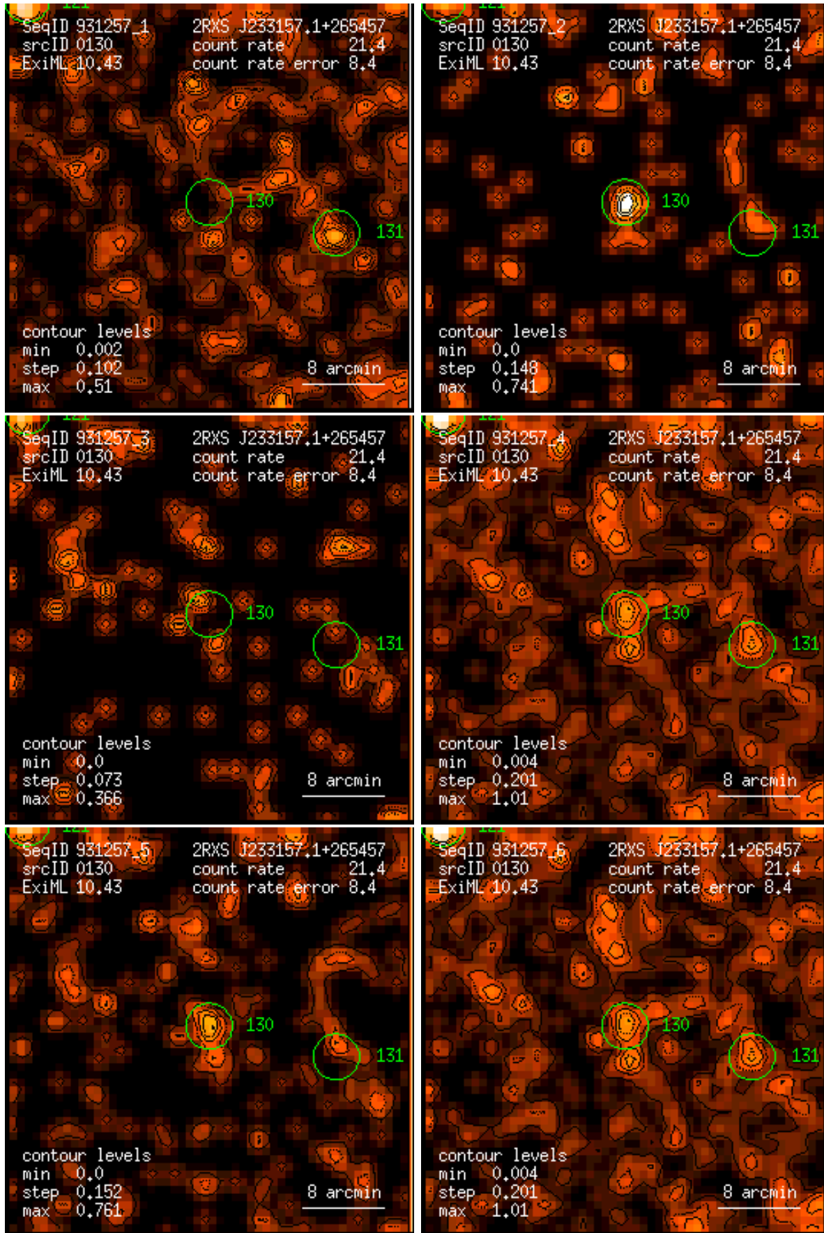
Figure 130: RASS 931257: detection 0130: band rate images, Gaussian filter: (1) PSPC channels 11 – 41, (2) 52 – 90, (3) 91 – 201, (4) 11 – 235, (5) 52 – 201, (6) 11 – 201. Broad band rates in counts/ks. Band rate contour levels in counts/ks/arcmin 2 .
