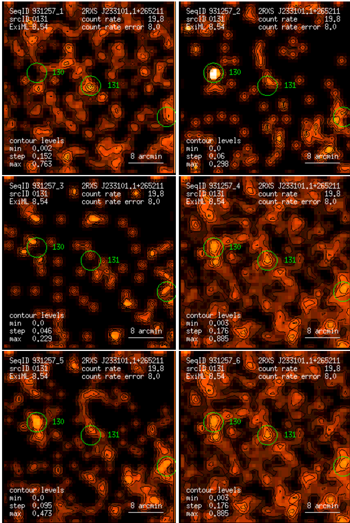
Figure 131: RASS 931257: detection 0131: band rate images, Gaussian filter: (1) PSPC channels 11 – 41, (2) 52 – 90, (3) 91 – 201, (4) 11 – 235, (5) 52 – 201, (6) 11 – 201. Broad band rates in counts/ks. Band rate contour levels in counts/ks/arcmin 2 .
