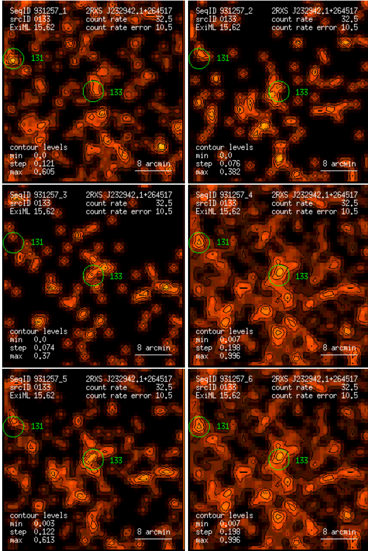
Figure 133: RASS 931257: detection 0133: band rate images, Gaussian filter: (1) PSPC channels 11 – 41, (2) 52 – 90, (3) 91 – 201, (4) 11 – 235, (5) 52 – 201, (6) 11 – 201. Broad band rates in counts/ks. Band rate contour levels in counts/ks/arcmin 2 .
