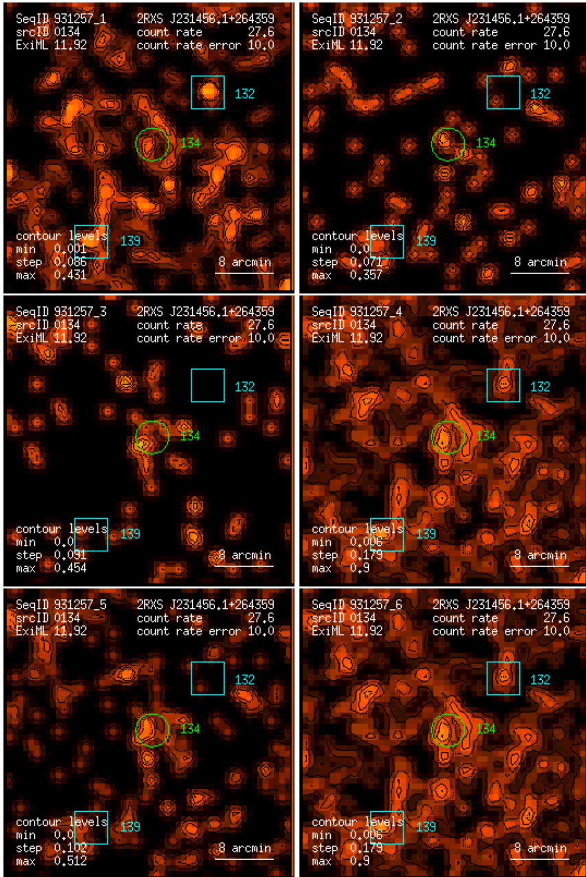
Figure 134: RASS 931257: detection 0134: band rate images, Gaussian filter: (1) PSPC channels 11 – 41, (2) 52 – 90, (3) 91 – 201, (4) 11 – 235, (5) 52 – 201, (6) 11 – 201. Broad band rates in counts/ks. Band rate contour levels in counts/ks/arcmin 2 .
