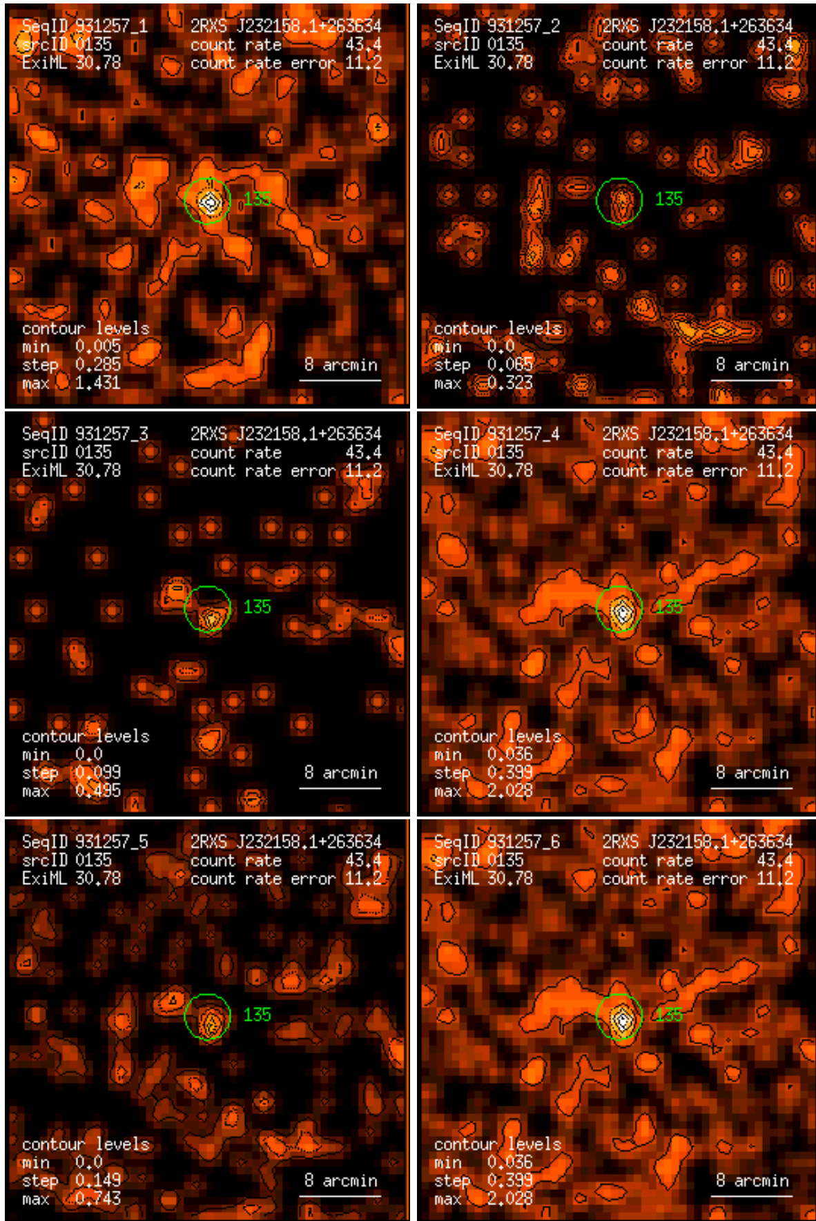
Figure 135: RASS 931257: detection 0135: band rate images, Gaussian filter: (1) PSPC channels 11 – 41, (2) 52 – 90, (3) 91 – 201, (4) 11 – 235, (5) 52 – 201, (6) 11 – 201. Broad band rates in counts/ks. Band rate contour levels in counts/ks/arcmin 2 .
