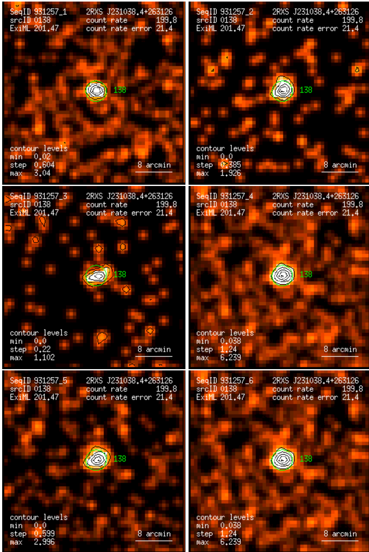
Figure 138: RASS 931257: detection 0138: band rate images, Gaussian filter: (1) PSPC channels 11 – 41, (2) 52 – 90, (3) 91 – 201, (4) 11 – 235, (5) 52 – 201, (6) 11 – 201. Broad band rates in counts/ks. Band rate contour levels in counts/ks/arcmin 2 .
