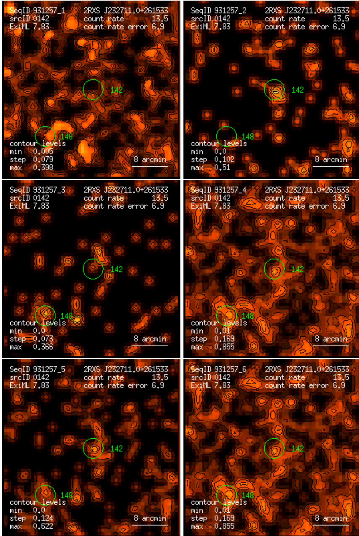
Figure 142: RASS 931257: detection 0142: band rate images, Gaussian filter: (1) PSPC channels 11 – 41, (2) 52 – 90, (3) 91 – 201, (4) 11 – 235, (5) 52 – 201, (6) 11 – 201. Broad band rates in counts/ks. Band rate contour levels in counts/ks/arcmin 2 .
