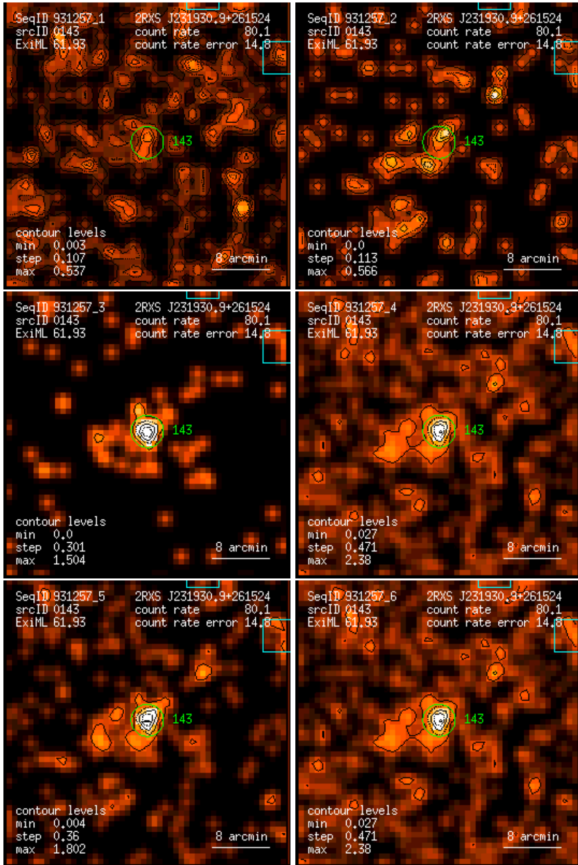
Figure 143: RASS 931257: detection 0143: band rate images, Gaussian filter: (1) PSPC channels 11 – 41, (2) 52 – 90, (3) 91 – 201, (4) 11 – 235, (5) 52 – 201, (6) 11 – 201. Broad band rates in counts/ks. Band rate contour levels in counts/ks/arcmin 2 .
