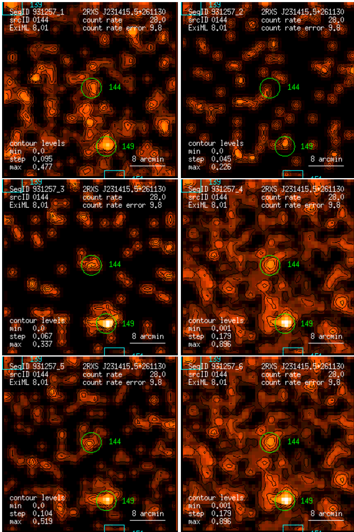
Figure 144: RASS 931257: detection 0144: band rate images, Gaussian filter: (1) PSPC channels 11 – 41, (2) 52 – 90, (3) 91 – 201, (4) 11 – 235, (5) 52 – 201, (6) 11 – 201. Broad band rates in counts/ks. Band rate contour levels in counts/ks/arcmin 2 .
