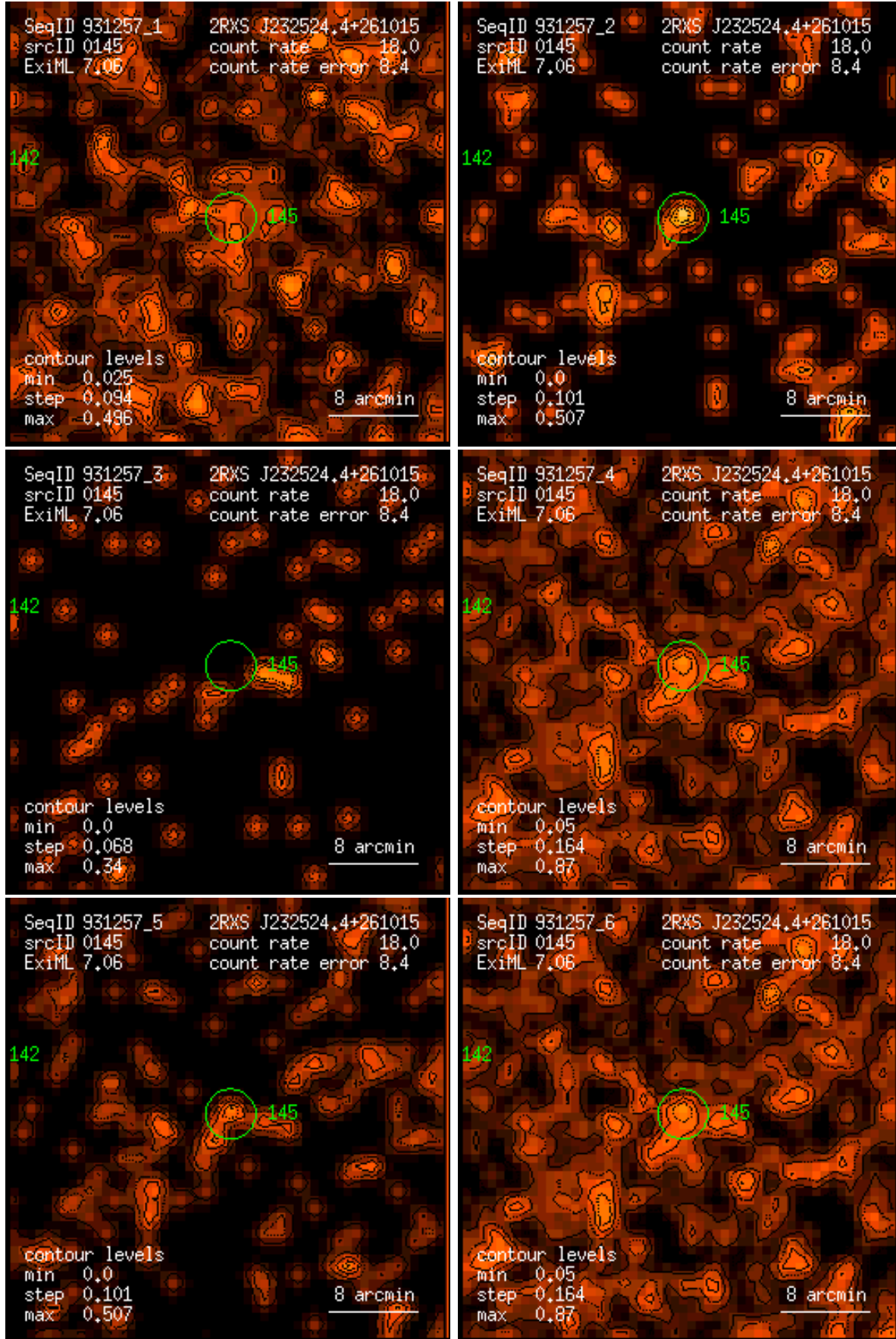
Figure 145: RASS 931257: detection 0145: band rate images, Gaussian filter: (1) PSPC channels 11 – 41, (2) 52 – 90, (3) 91 – 201, (4) 11 – 235, (5) 52 – 201, (6) 11 – 201. Broad band rates in counts/ks. Band rate contour levels in counts/ks/arcmin 2 .
