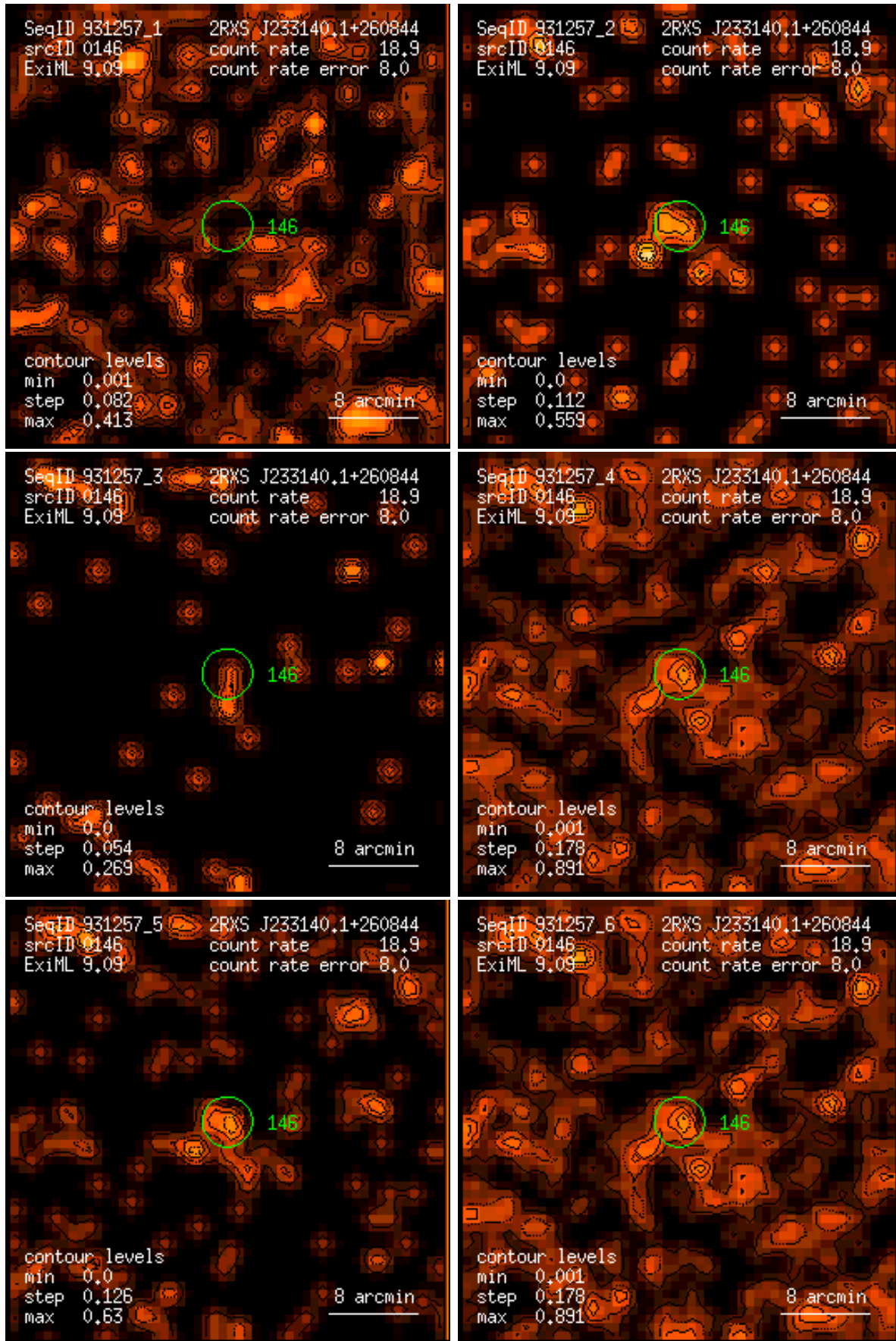
Figure 146: RASS 931257: detection 0146: band rate images, Gaussian filter: (1) PSPC channels 11 – 41, (2) 52 – 90, (3) 91 – 201, (4) 11 – 235, (5) 52 – 201, (6) 11 – 201. Broad band rates in counts/ks. Band rate contour levels in counts/ks/arcmin 2 .
