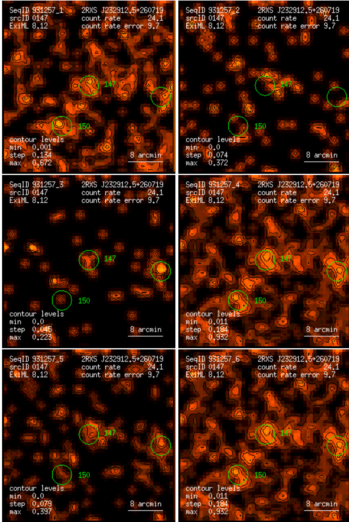
Figure 147: RASS 931257: detection 0147: band rate images, Gaussian filter: (1) PSPC channels 11 – 41, (2) 52 – 90, (3) 91 – 201, (4) 11 – 235, (5) 52 – 201, (6) 11 – 201. Broad band rates in counts/ks. Band rate contour levels in counts/ks/arcmin 2 .
