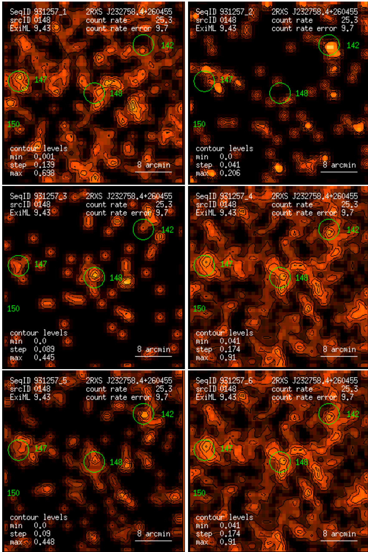
Figure 148: RASS 931257: detection 0148: band rate images, Gaussian filter: (1) PSPC channels 11 – 41, (2) 52 – 90, (3) 91 – 201, (4) 11 – 235, (5) 52 – 201, (6) 11 – 201. Broad band rates in counts/ks. Band rate contour levels in counts/ks/arcmin 2 .
