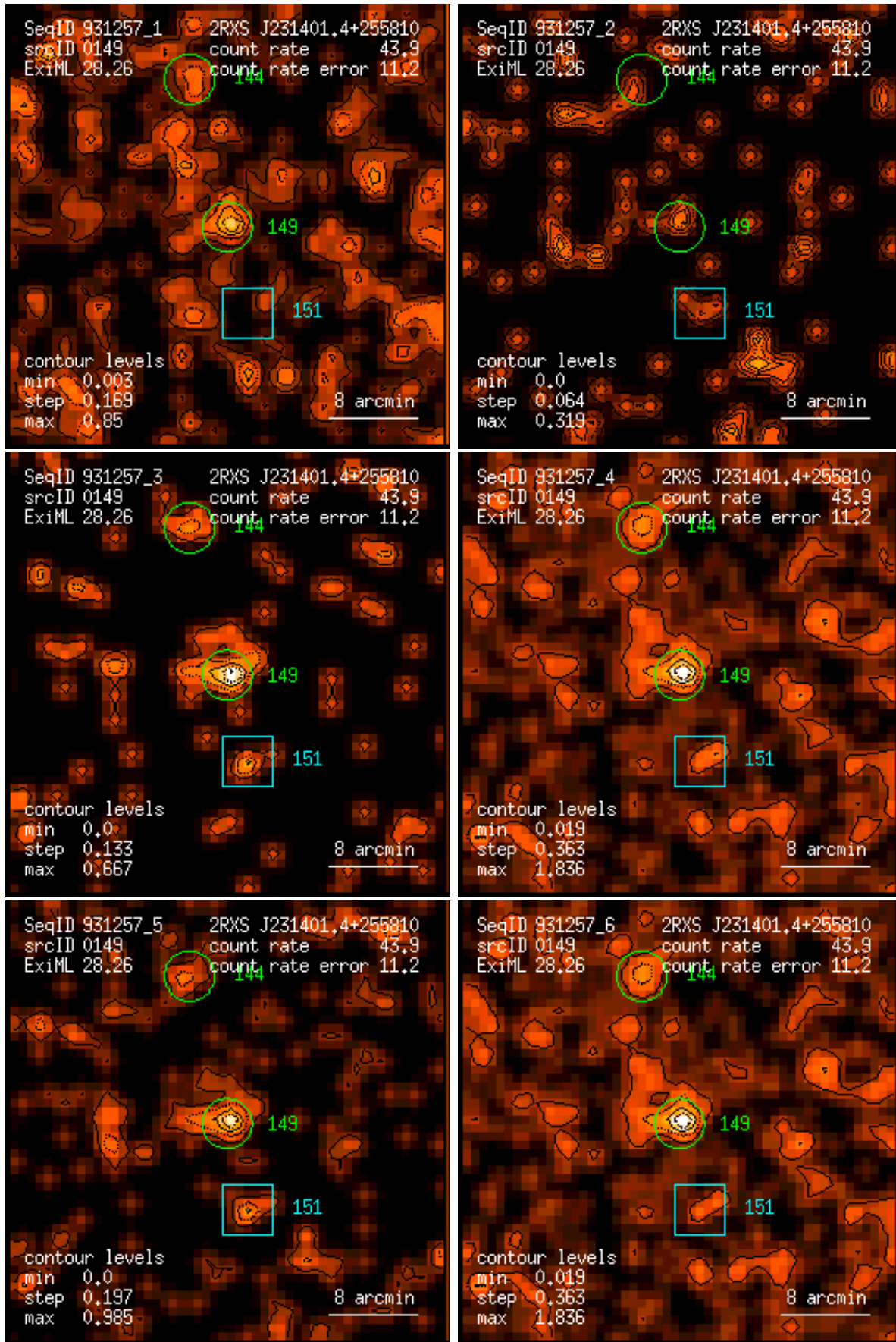
Figure 149: RASS 931257: detection 0149: band rate images, Gaussian filter: (1) PSPC channels 11 – 41, (2) 52 – 90, (3) 91 – 201, (4) 11 – 235, (5) 52 – 201, (6) 11 – 201. Broad band rates in counts/ks. Band rate contour levels in counts/ks/arcmin 2 .
