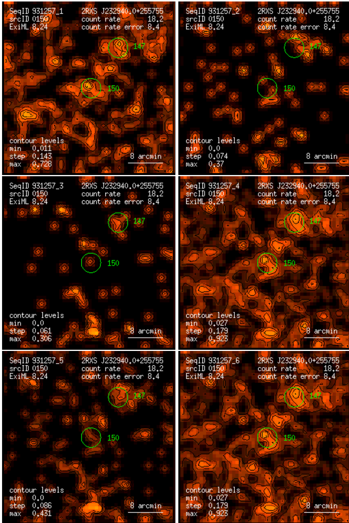
Figure 150: RASS 931257: detection 0150: band rate images, Gaussian filter: (1) PSPC channels 11 – 41, (2) 52 – 90, (3) 91 – 201, (4) 11 – 235, (5) 52 – 201, (6) 11 – 201. Broad band rates in counts/ks. Band rate contour levels in counts/ks/arcmin 2 .
