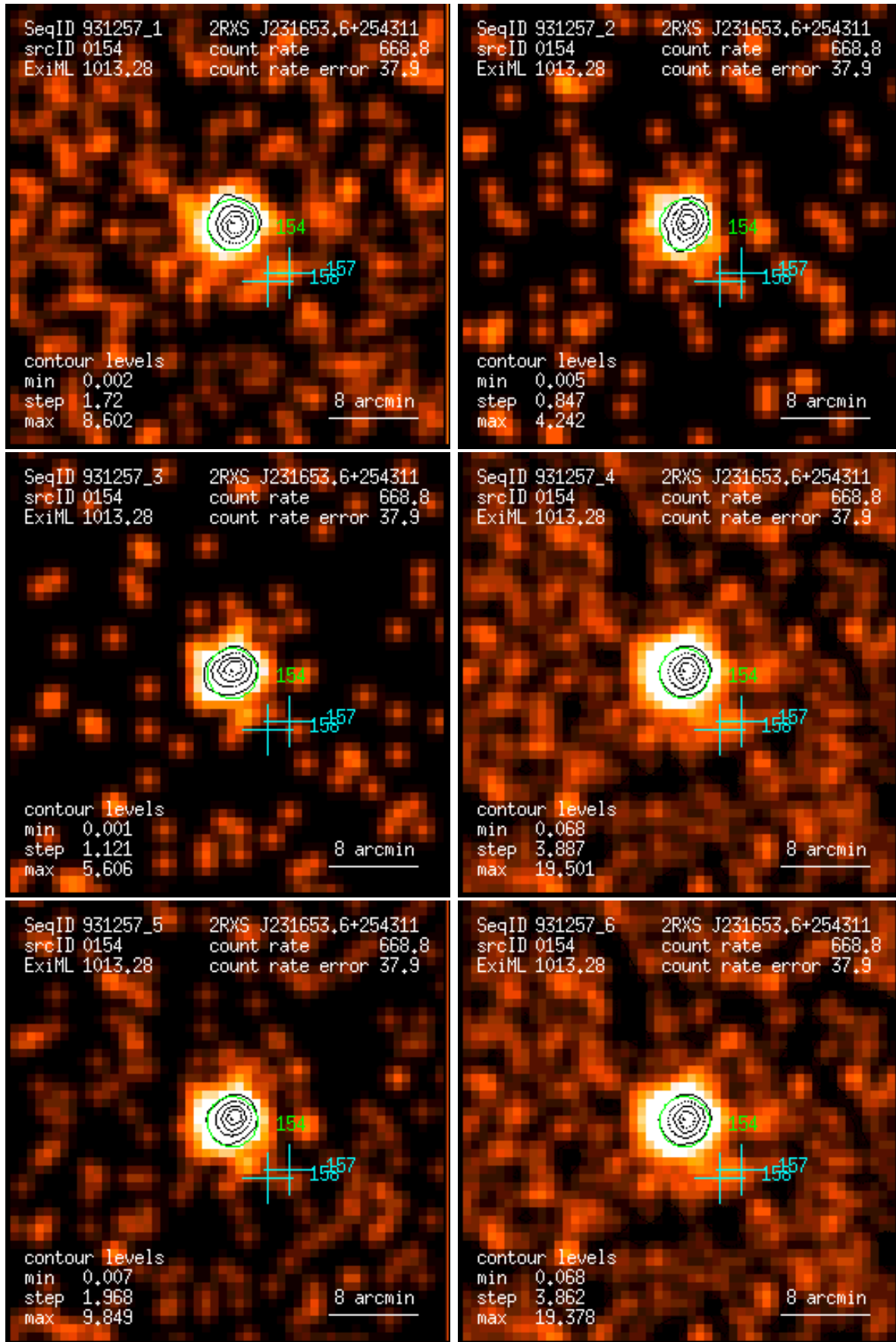
Figure 154: RASS 931257: detection 0154: band rate images, Gaussian filter: (1) PSPC channels 11 – 41, (2) 52 – 90, (3) 91 – 201, (4) 11 – 235, (5) 52 – 201, (6) 11 – 201. Broad band rates in counts/ks. Band rate contour levels in counts/ks/arcmin 2 .
