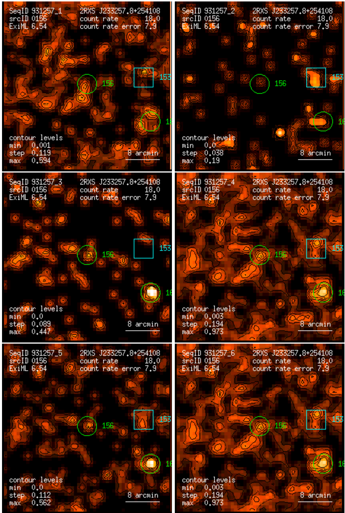
Figure 156: RASS 931257: detection 0156: band rate images, Gaussian filter: (1) PSPC channels 11 – 41, (2) 52 – 90, (3) 91 – 201, (4) 11 – 235, (5) 52 – 201, (6) 11 – 201. Broad band rates in counts/ks. Band rate contour levels in counts/ks/arcmin 2 .
