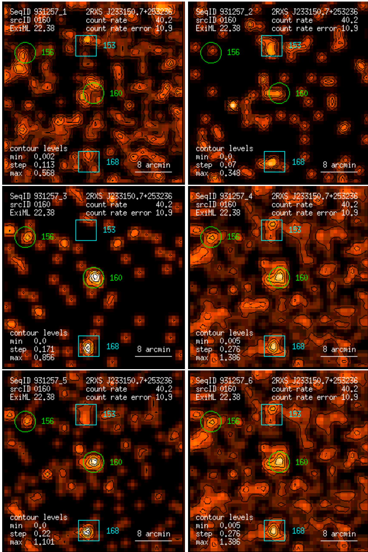
Figure 160: RASS 931257: detection 0160: band rate images, Gaussian filter: (1) PSPC channels 11 – 41, (2) 52 – 90, (3) 91 – 201, (4) 11 – 235, (5) 52 – 201, (6) 11 – 201. Broad band rates in counts/ks. Band rate contour levels in counts/ks/arcmin 2 .
