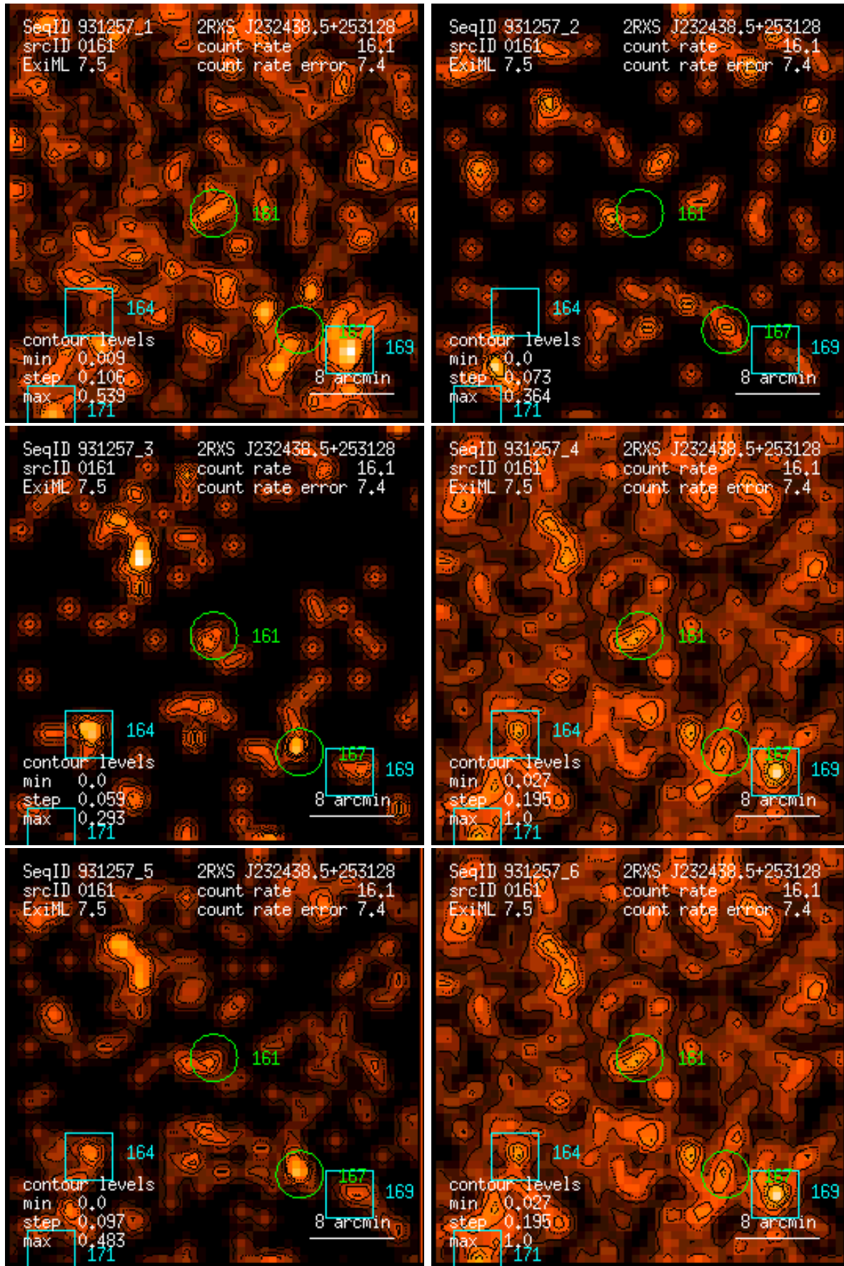
Figure 161: RASS 931257: detection 0161: band rate images, Gaussian filter: (1) PSPC channels 11 – 41, (2) 52 – 90, (3) 91 – 201, (4) 11 – 235, (5) 52 – 201, (6) 11 – 201. Broad band rates in counts/ks. Band rate contour levels in counts/ks/arcmin 2 .
