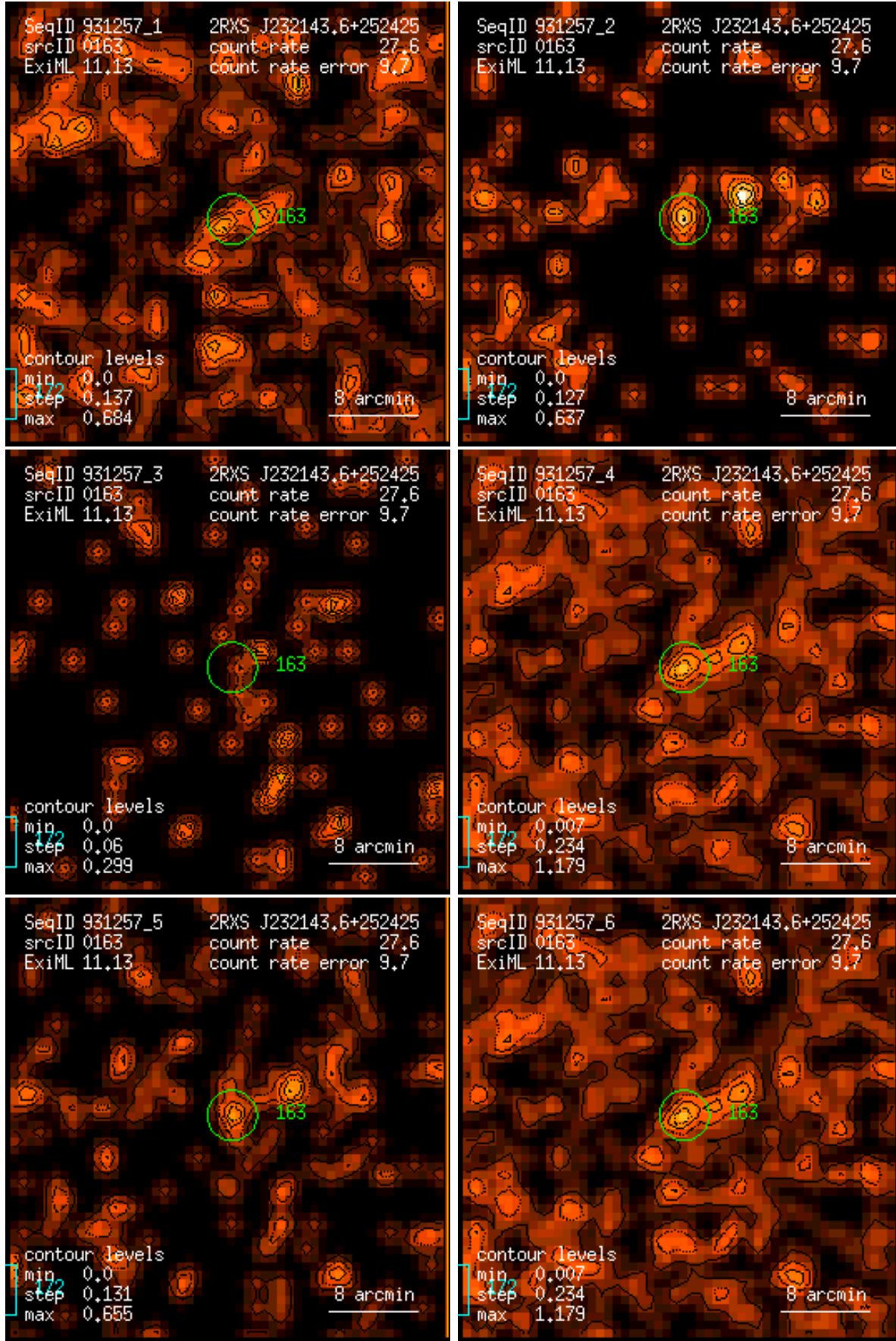
Figure 163: RASS 931257: detection 0163: band rate images, Gaussian filter: (1) PSPC channels 11 – 41, (2) 52 – 90, (3) 91 – 201, (4) 11 – 235, (5) 52 – 201, (6) 11 – 201. Broad band rates in counts/ks. Band rate contour levels in counts/ks/arcmin 2 .
