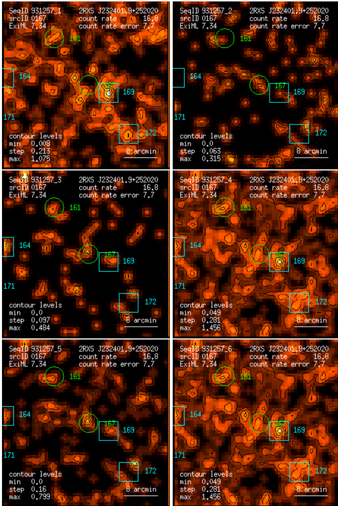
Figure 167: RASS 931257: detection 0167: band rate images, Gaussian filter: (1) PSPC channels 11 – 41, (2) 52 – 90, (3) 91 – 201, (4) 11 – 235, (5) 52 – 201, (6) 11 – 201. Broad band rates in counts/ks. Band rate contour levels in counts/ks/arcmin 2 .
