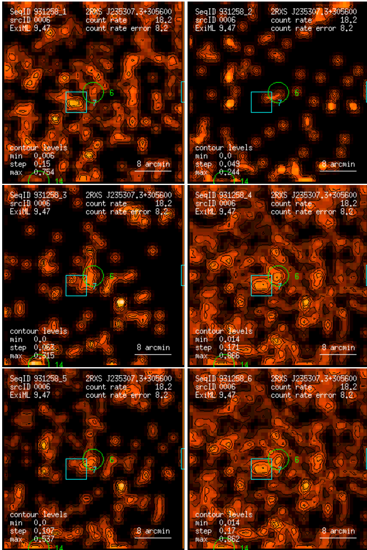
Figure 6: RASS 931258: detection 0006: band rate images, Gaussian filter: (1) PSPC channels 11 – 41, (2) 52 – 90, (3) 91 – 201, (4) 11 – 235, (5) 52 – 201, (6) 11 – 201. Broad band rates in counts/ks. Band rate contour levels in counts/ks/arcmin 2 .
