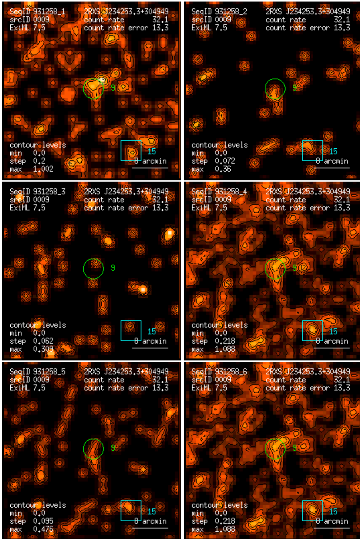
Figure 9: RASS 931258: detection 0009: band rate images, Gaussian filter: (1) PSPC channels 11 – 41, (2) 52 – 90, (3) 91 – 201, (4) 11 – 235, (5) 52 – 201, (6) 11 – 201. Broad band rates in counts/ks. Band rate contour levels in counts/ks/arcmin 2 .
