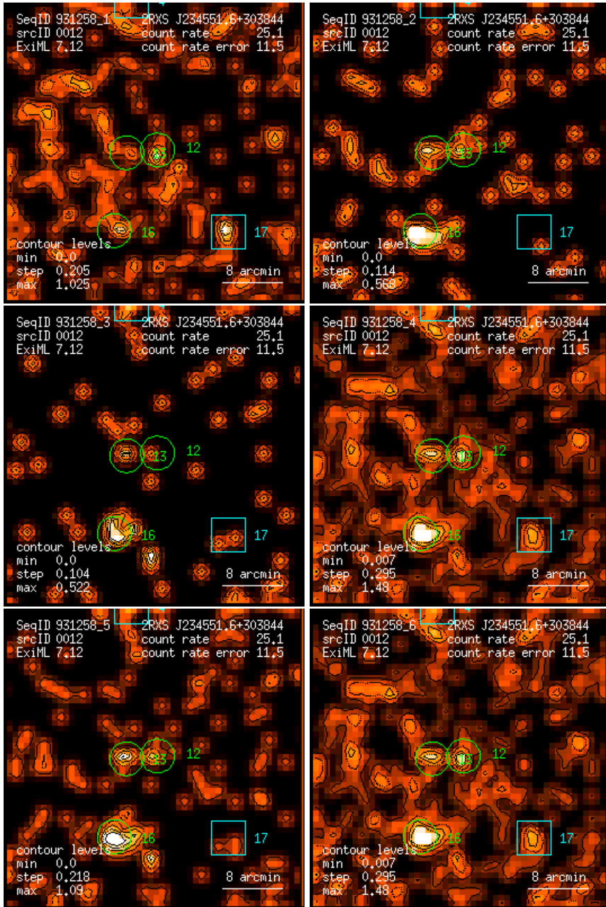
Figure 12: RASS 931258: detection 0012: band rate images, Gaussian filter: (1) PSPC channels 11 – 41, (2) 52 – 90, (3) 91 – 201, (4) 11 – 235, (5) 52 – 201, (6) 11 – 201. Broad band rates in counts/ks. Band rate contour levels in counts/ks/arcmin 2 .
