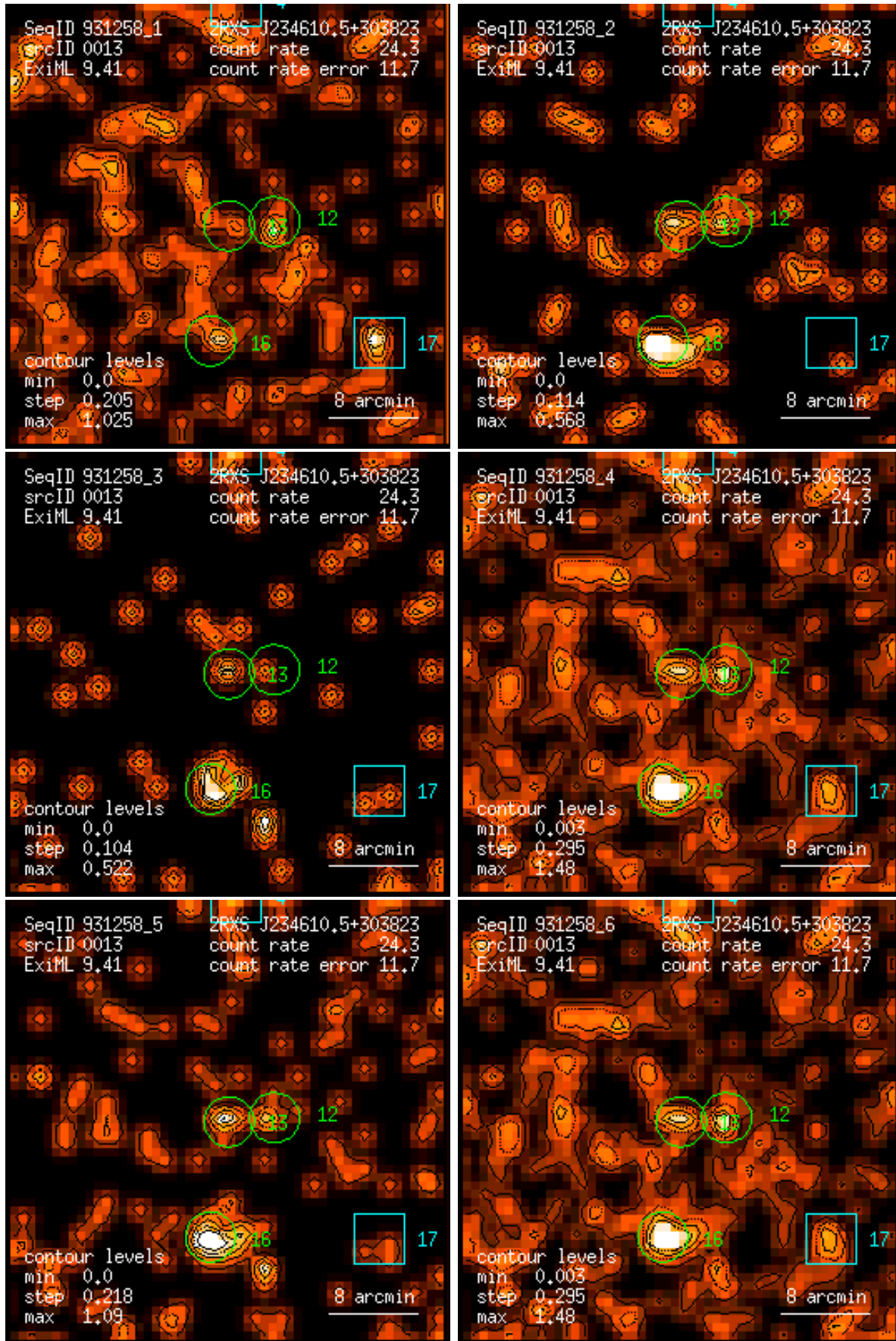
Figure 13: RASS 931258: detection 0013: band rate images, Gaussian filter: (1) PSPC channels 11 – 41, (2) 52 – 90, (3) 91 – 201, (4) 11 – 235, (5) 52 – 201, (6) 11 – 201. Broad band rates in counts/ks. Band rate contour levels in counts/ks/arcmin 2 .
