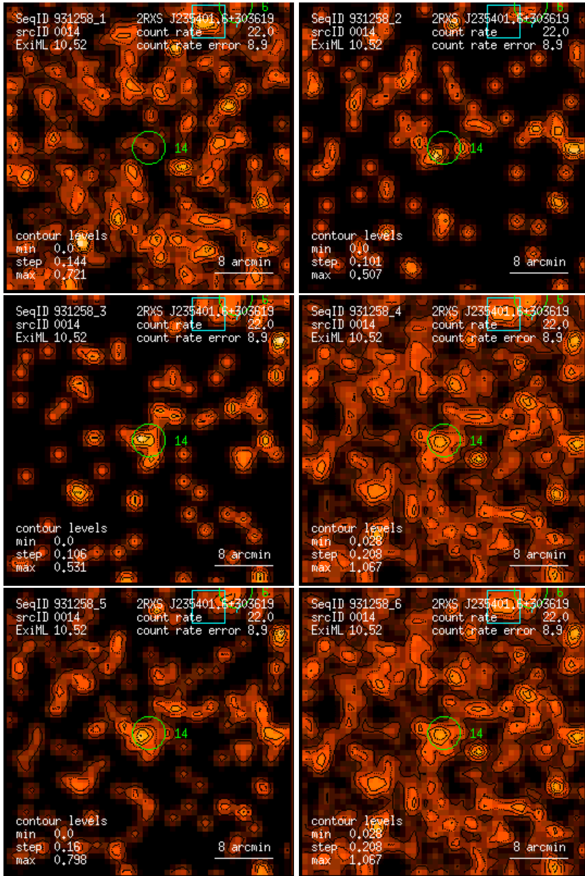
Figure 14: RASS 931258: detection 0014: band rate images, Gaussian filter: (1) PSPC channels 11 – 41, (2) 52 – 90, (3) 91 – 201, (4) 11 – 235, (5) 52 – 201, (6) 11 – 201. Broad band rates in counts/ks. Band rate contour levels in counts/ks/arcmin 2 .
