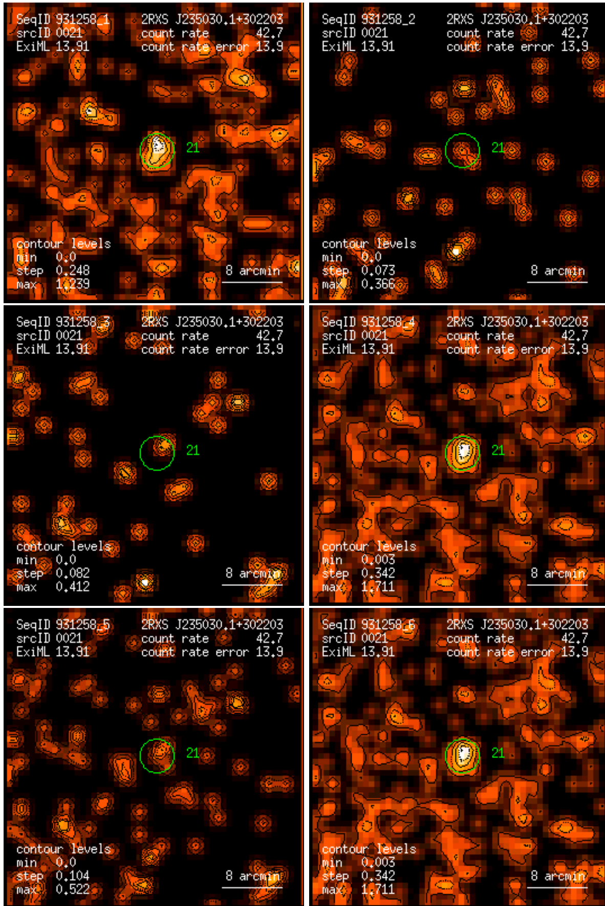
Figure 21: RASS 931258: detection 0021: band rate images, Gaussian filter: (1) PSPC channels 11 – 41, (2) 52 – 90, (3) 91 – 201, (4) 11 – 235, (5) 52 – 201, (6) 11 – 201. Broad band rates in counts/ks. Band rate contour levels in counts/ks/arcmin 2 .
