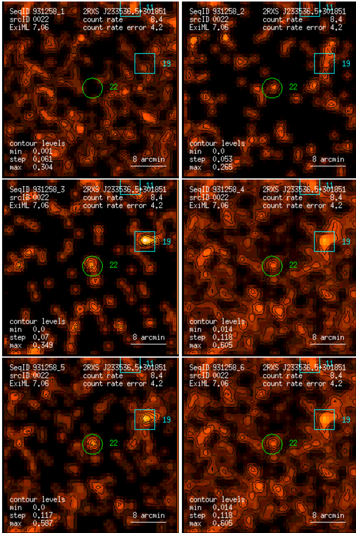
Figure 22: RASS 931258: detection 0022: band rate images, Gaussian filter: (1) PSPC channels 11 – 41, (2) 52 – 90, (3) 91 – 201, (4) 11 – 235, (5) 52 – 201, (6) 11 – 201. Broad band rates in counts/ks. Band rate contour levels in counts/ks/arcmin 2 .
