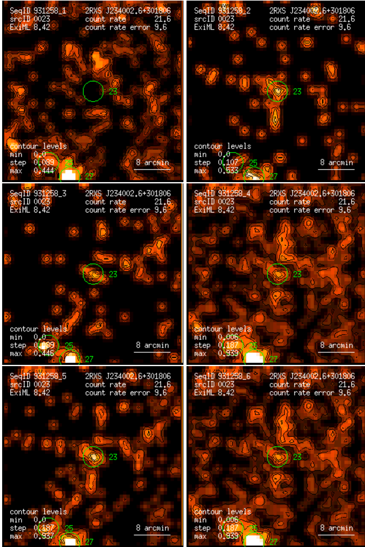
Figure 23: RASS 931258: detection 0023: band rate images, Gaussian filter: (1) PSPC channels 11 – 41, (2) 52 – 90, (3) 91 – 201, (4) 11 – 235, (5) 52 – 201, (6) 11 – 201. Broad band rates in counts/ks. Band rate contour levels in counts/ks/arcmin 2 .
