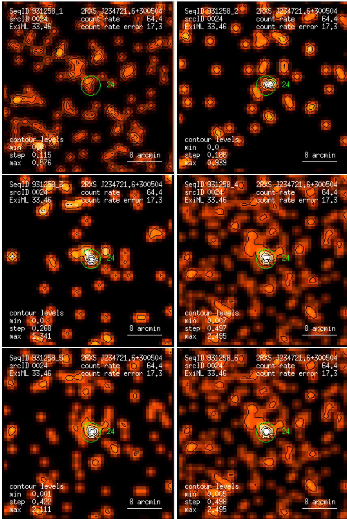
Figure 24: RASS 931258: detection 0024: band rate images, Gaussian filter: (1) PSPC channels 11 – 41, (2) 52 – 90, (3) 91 – 201, (4) 11 – 235, (5) 52 – 201, (6) 11 – 201. Broad band rates in counts/ks. Band rate contour levels in counts/ks/arcmin 2 .
