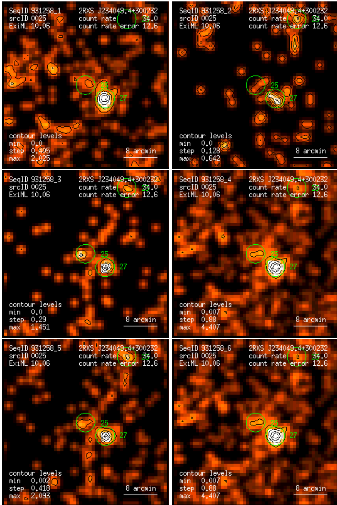
Figure 25: RASS 931258: detection 0025: band rate images, Gaussian filter: (1) PSPC channels 11 – 41, (2) 52 – 90, (3) 91 – 201, (4) 11 – 235, (5) 52 – 201, (6) 11 – 201. Broad band rates in counts/ks. Band rate contour levels in counts/ks/arcmin 2 .
