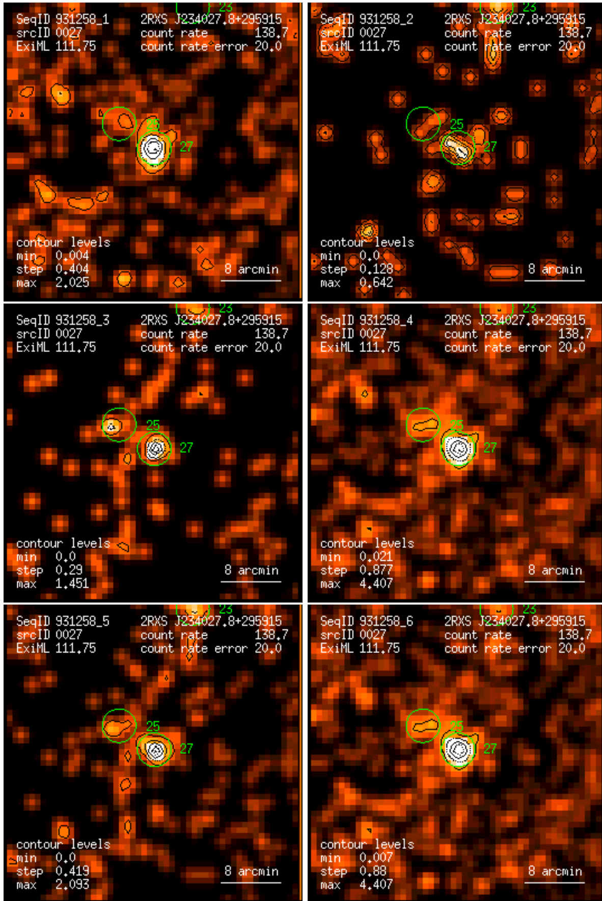
Figure 27: RASS 931258: detection 0027: band rate images, Gaussian filter: (1) PSPC channels 11 – 41, (2) 52 – 90, (3) 91 – 201, (4) 11 – 235, (5) 52 – 201, (6) 11 – 201. Broad band rates in counts/ks. Band rate contour levels in counts/ks/arcmin 2 .
