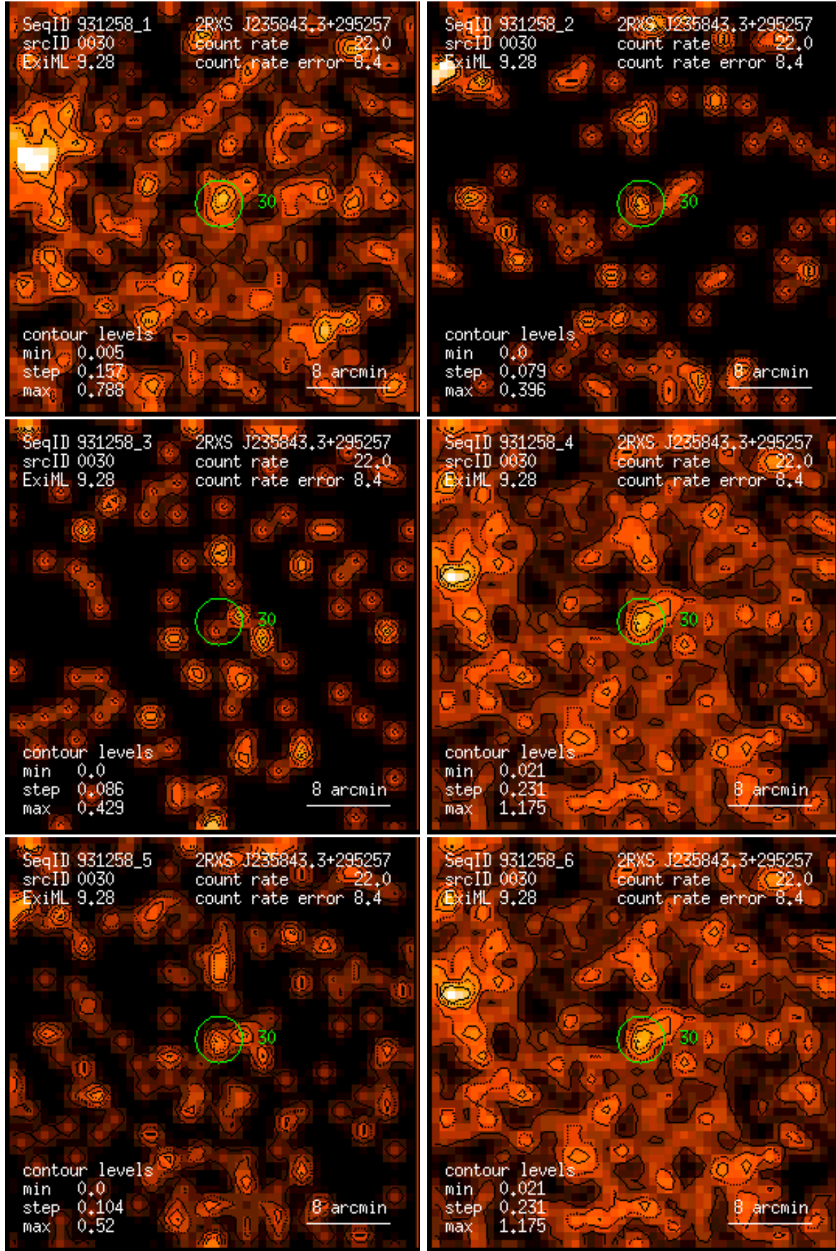
Figure 30: RASS 931258: detection 0030: band rate images, Gaussian filter: (1) PSPC channels 11 – 41, (2) 52 – 90, (3) 91 – 201, (4) 11 – 235, (5) 52 – 201, (6) 11 – 201. Broad band rates in counts/ks. Band rate contour levels in counts/ks/arcmin 2 .
