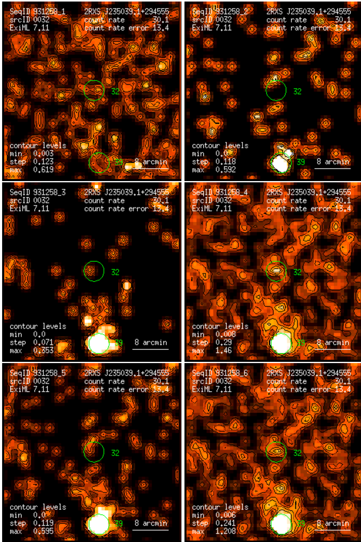
Figure 32: RASS 931258: detection 0032: band rate images, Gaussian filter: (1) PSPC channels 11 – 41, (2) 52 – 90, (3) 91 – 201, (4) 11 – 235, (5) 52 – 201, (6) 11 – 201. Broad band rates in counts/ks. Band rate contour levels in counts/ks/arcmin 2 .
