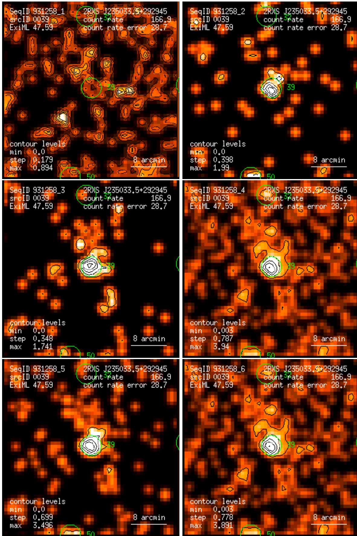
Figure 39: RASS 931258: detection 0039: band rate images, Gaussian filter: (1) PSPC channels 11 – 41, (2) 52 – 90, (3) 91 – 201, (4) 11 – 235, (5) 52 – 201, (6) 11 – 201. Broad band rates in counts/ks. Band rate contour levels in counts/ks/arcmin 2 .
