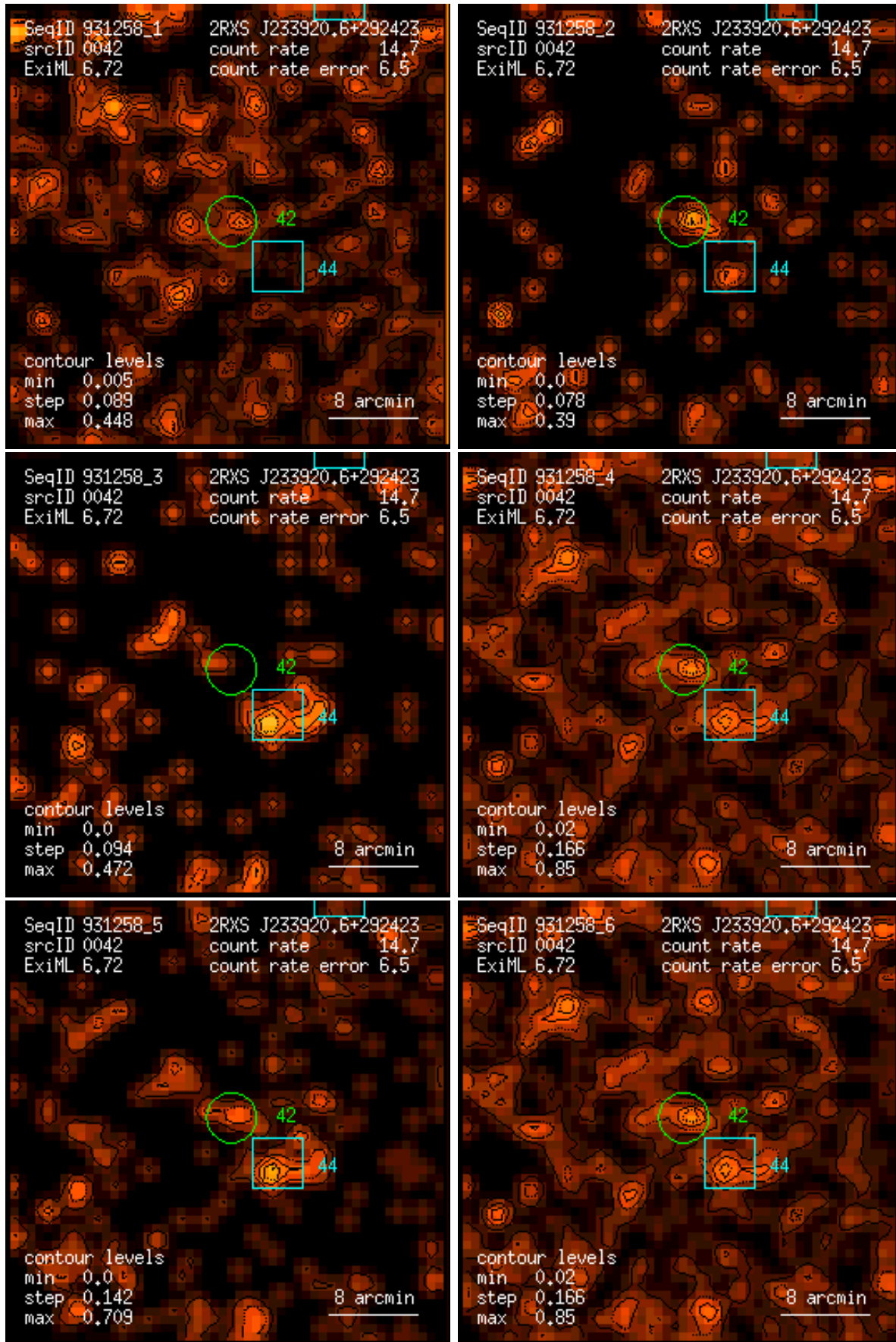
Figure 42: RASS 931258: detection 0042: band rate images, Gaussian filter: (1) PSPC channels 11 – 41, (2) 52 – 90, (3) 91 – 201, (4) 11 – 235, (5) 52 – 201, (6) 11 – 201. Broad band rates in counts/ks. Band rate contour levels in counts/ks/arcmin 2 .
