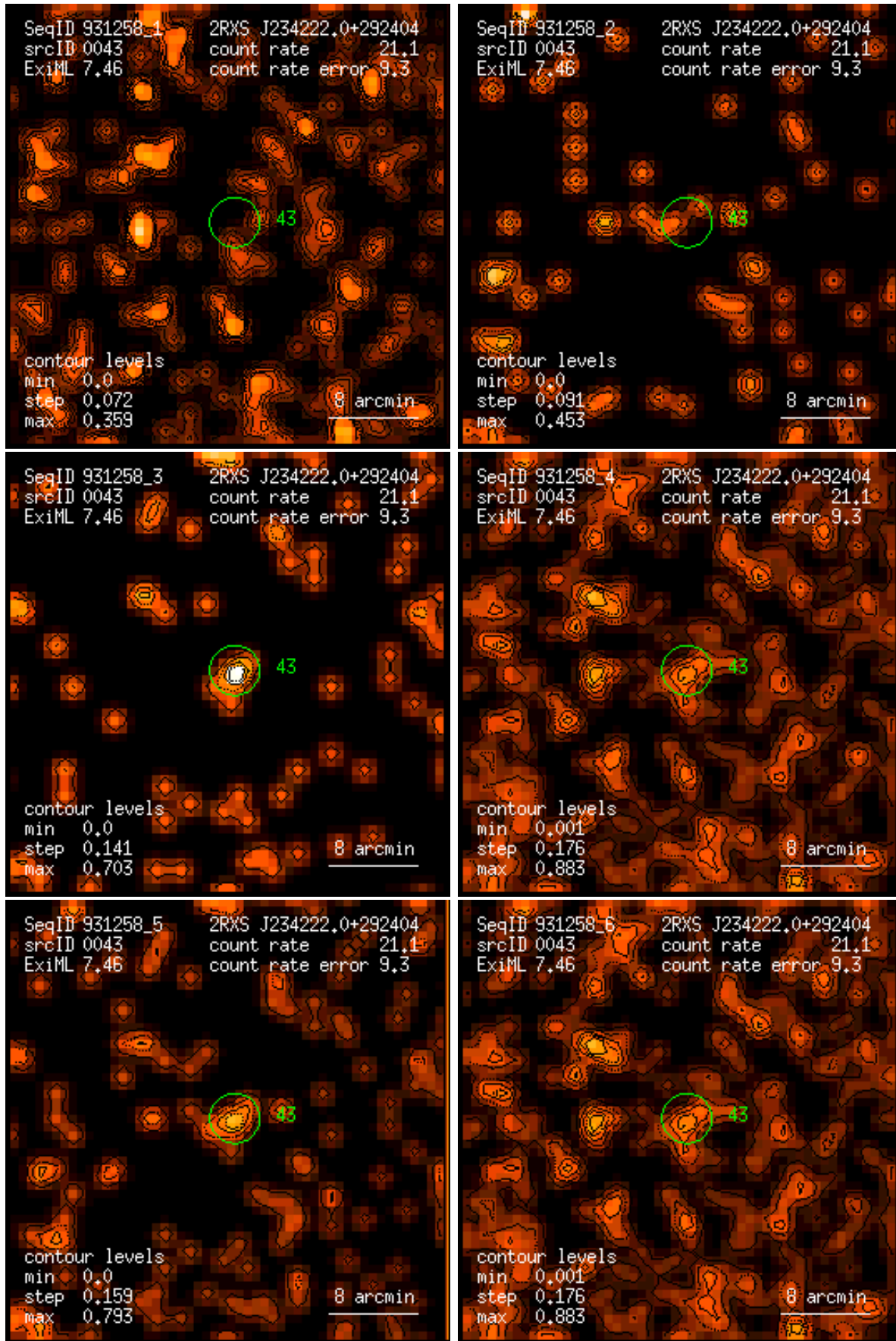
Figure 43: RASS 931258: detection 0043: band rate images, Gaussian filter: (1) PSPC channels 11 – 41, (2) 52 – 90, (3) 91 – 201, (4) 11 – 235, (5) 52 – 201, (6) 11 – 201. Broad band rates in counts/ks. Band rate contour levels in counts/ks/arcmin 2 .
